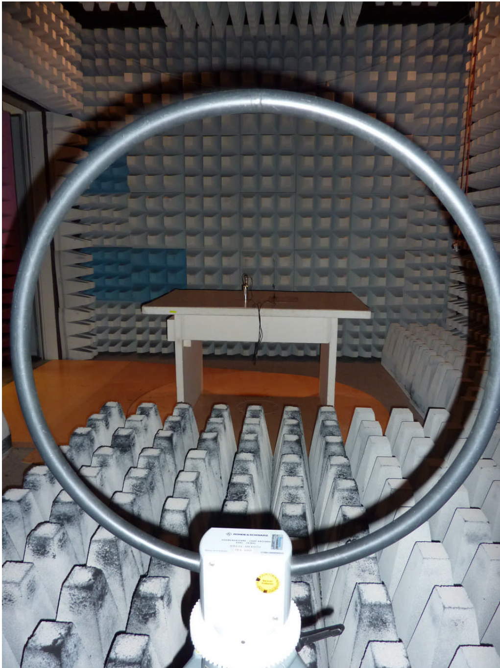
112414_8.JPG: Zonescan 820 Logger with external antenna, test setup fully anechoic chamber
