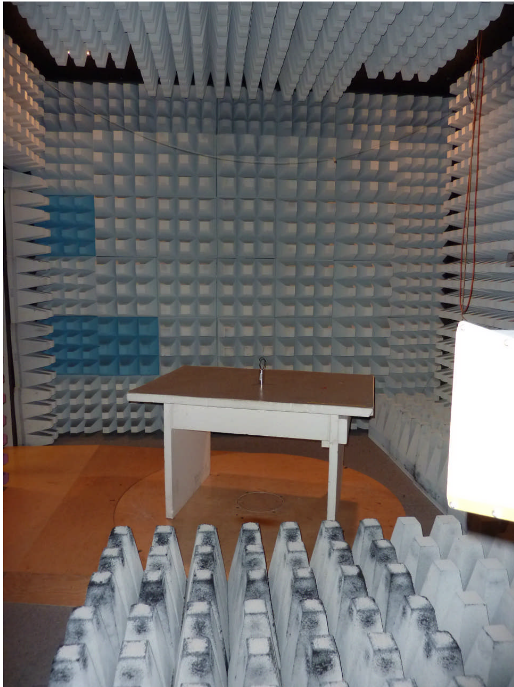
112414_7.JPG: Zonescan 820 Logger with external antenna, test setup fully anechoic chamber
