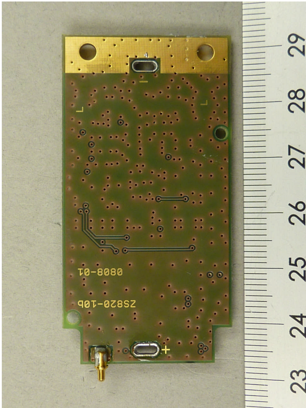
112414_f.JPG: Zonescan 820 Logger and Repeater, PCB, bottom view
