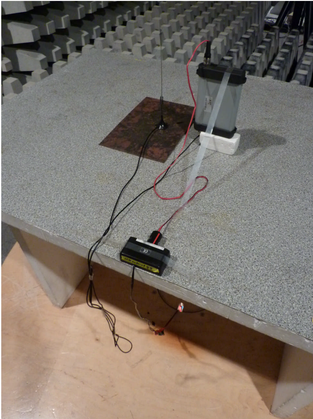
112416_10.JPG: Zonescan 820 Commlink, test set-up fully anechoic chamber (pos. 3)
