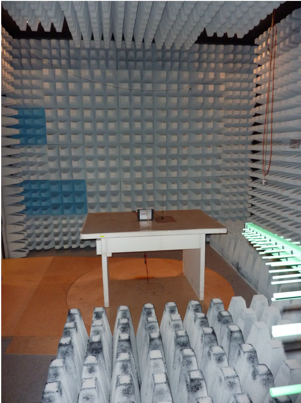
112416_3.JPG: Zonescan 820 Commlink, test set-up fully anechoic chamber (pos. 1)
