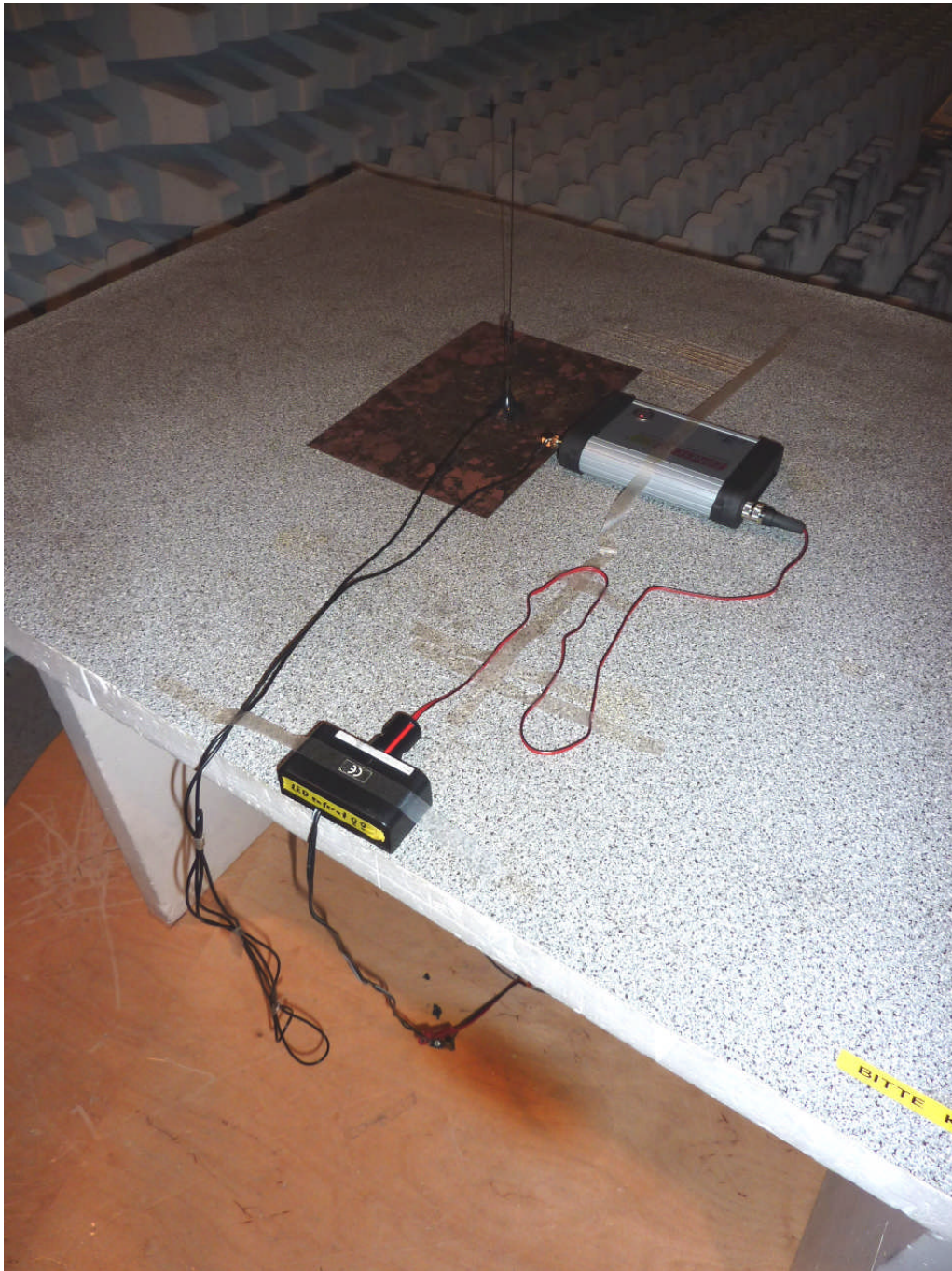
112416_7.JPG: Zonescan 820 Commlink, test set-up fully anechoic chamber (pos. 2)
