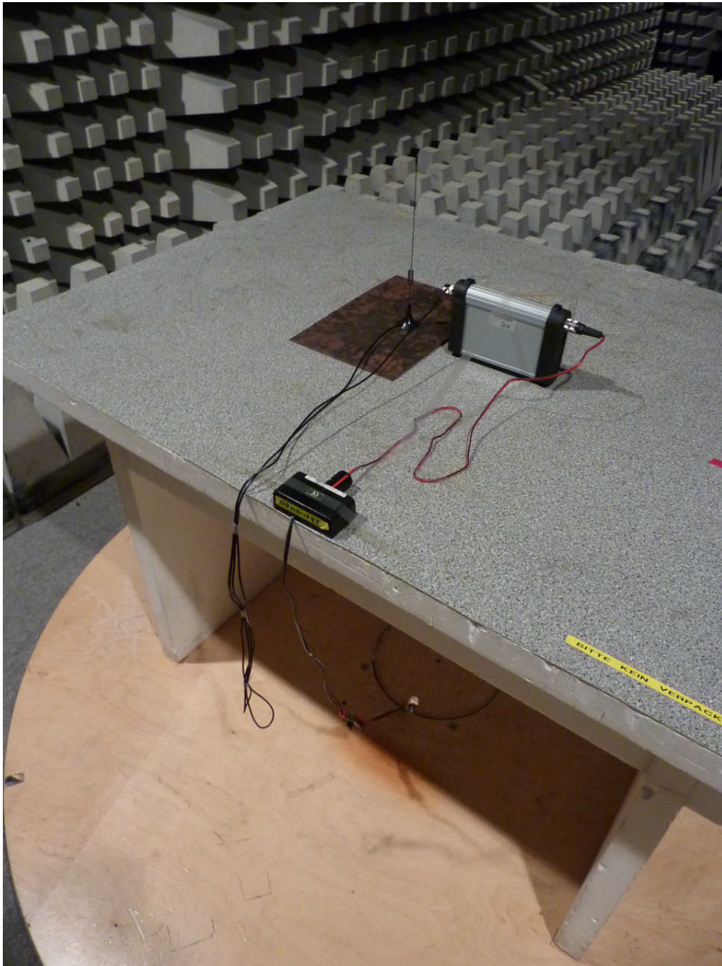
112416_1.JPG: Zonescan 820 Commlink, test set-up fully anechoic chamber (pos. 1)
