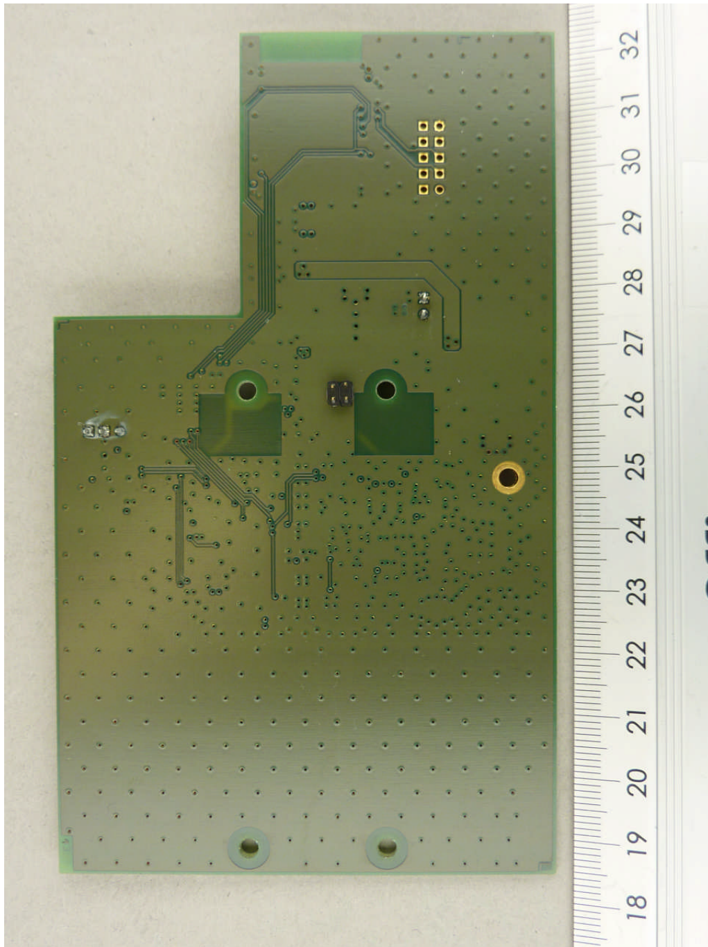
112416_g.JPG: Zonescan 820 Commlink, PCB, bottom view, battery removed
