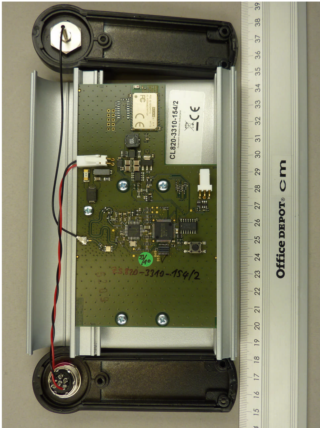
112416_d.JPG: Zonescan 820 Commlink, internal view
