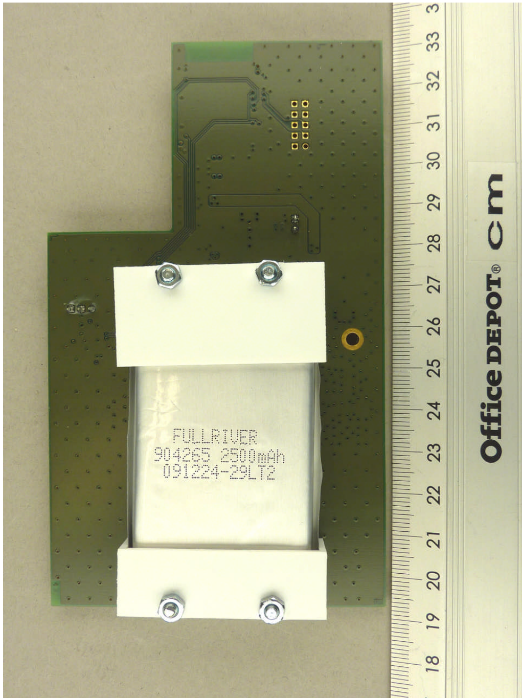
112416_f.JPG: Zonescan 820 Commlink, PCB, bottom view
