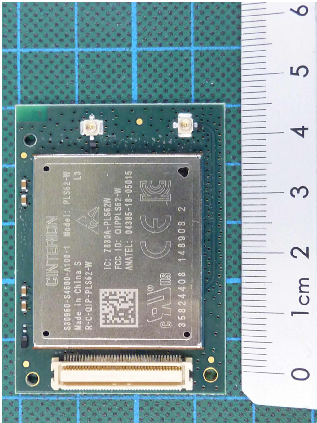
ZONESCAN 820 Alpha V2, cellular module, top view
