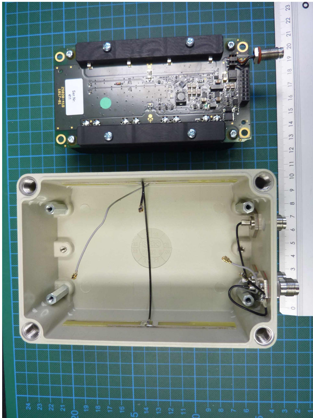
ZONESCAN 820 Alpha V2, internal view (battery PCB removed)
