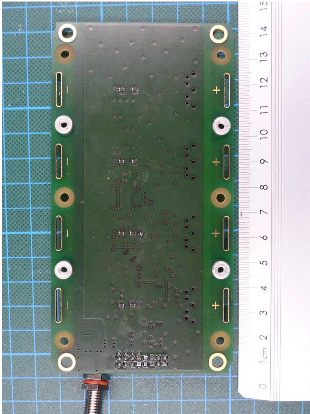
ZONESCAN 820 Alpha V2, battery PCB, bottom view (battery removed)
