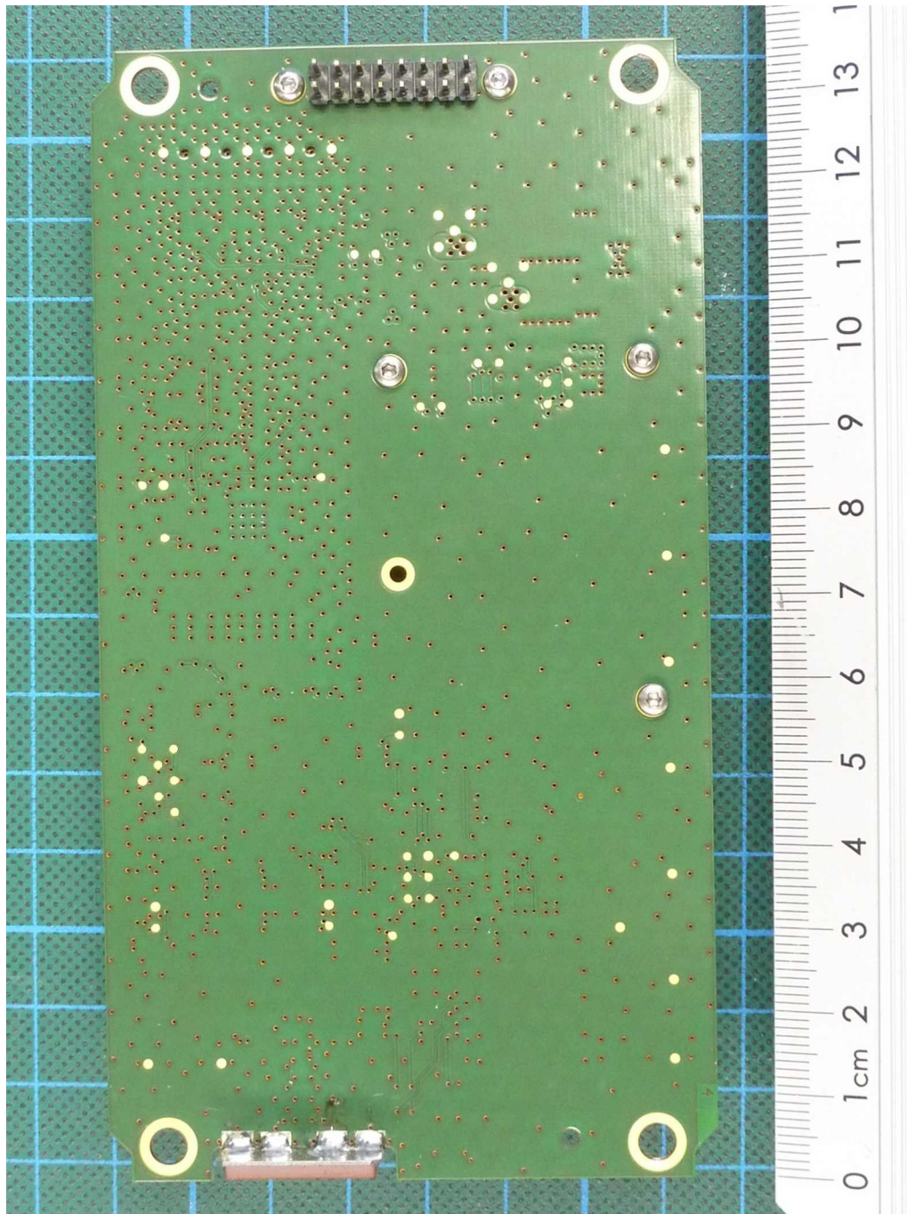
ZONESCAN 820 Alpha V2, main PCB, bottom view
