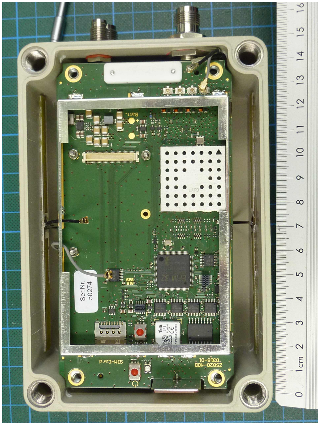
ZONESCAN 820 Alpha V2, internal view (cellular module removed)
