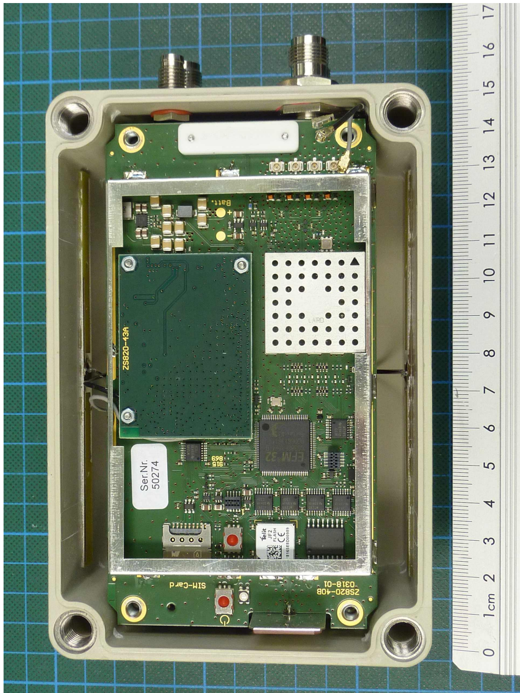
ZONESCAN 820 Alpha V2, internal view (shielding removed)
