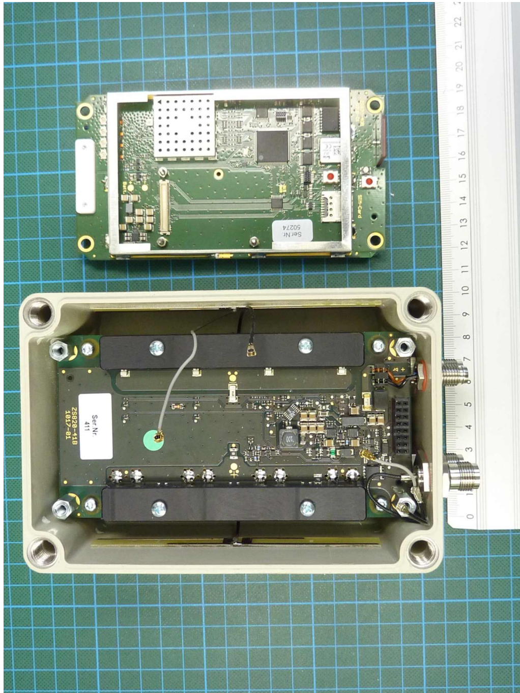
ZONESCAN 820 Alpha V2, internal view (main PCB removed)
