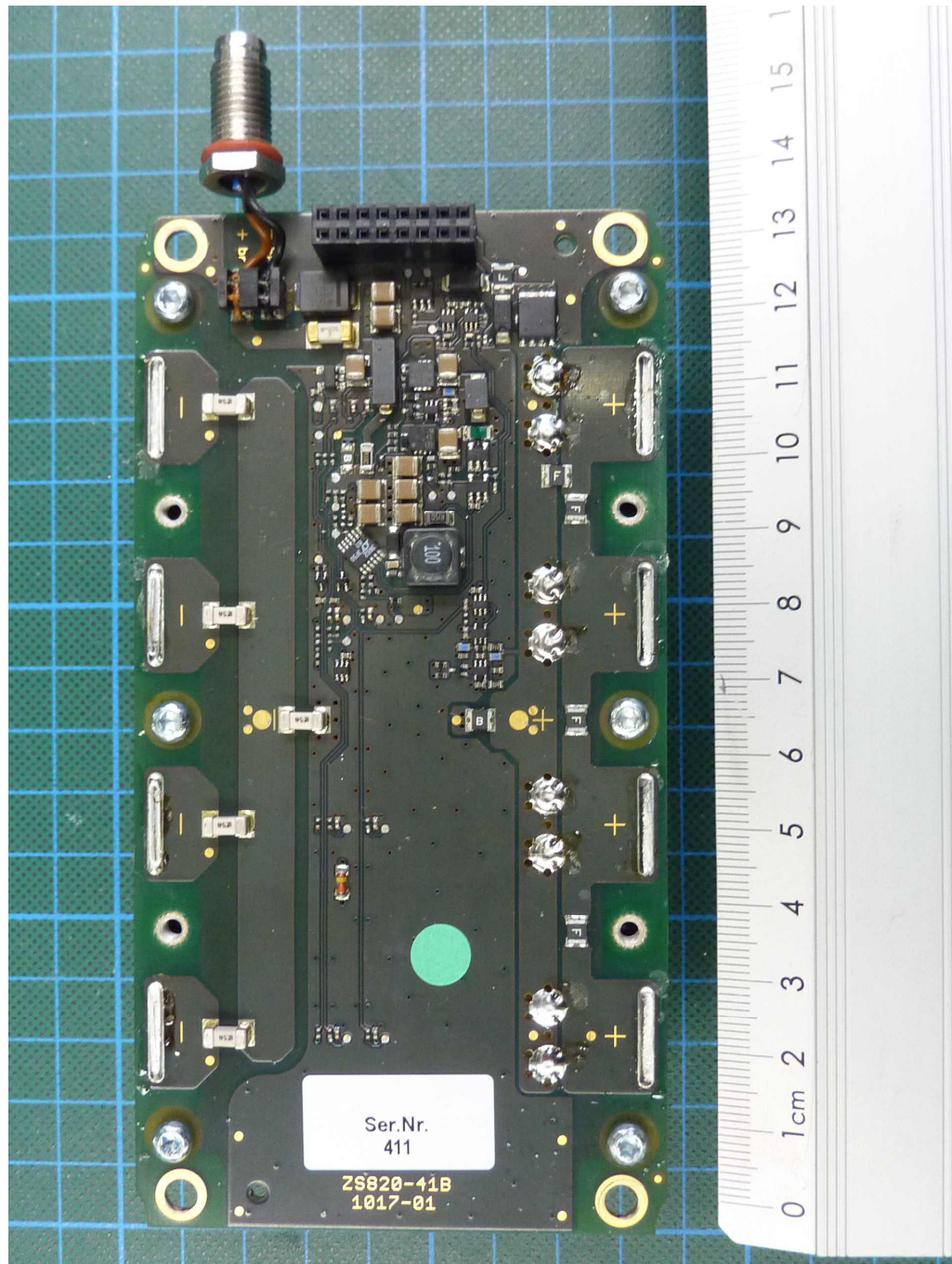
ZONESCAN 820 Alpha V2, battery PCB, top view (battery holder removed)
