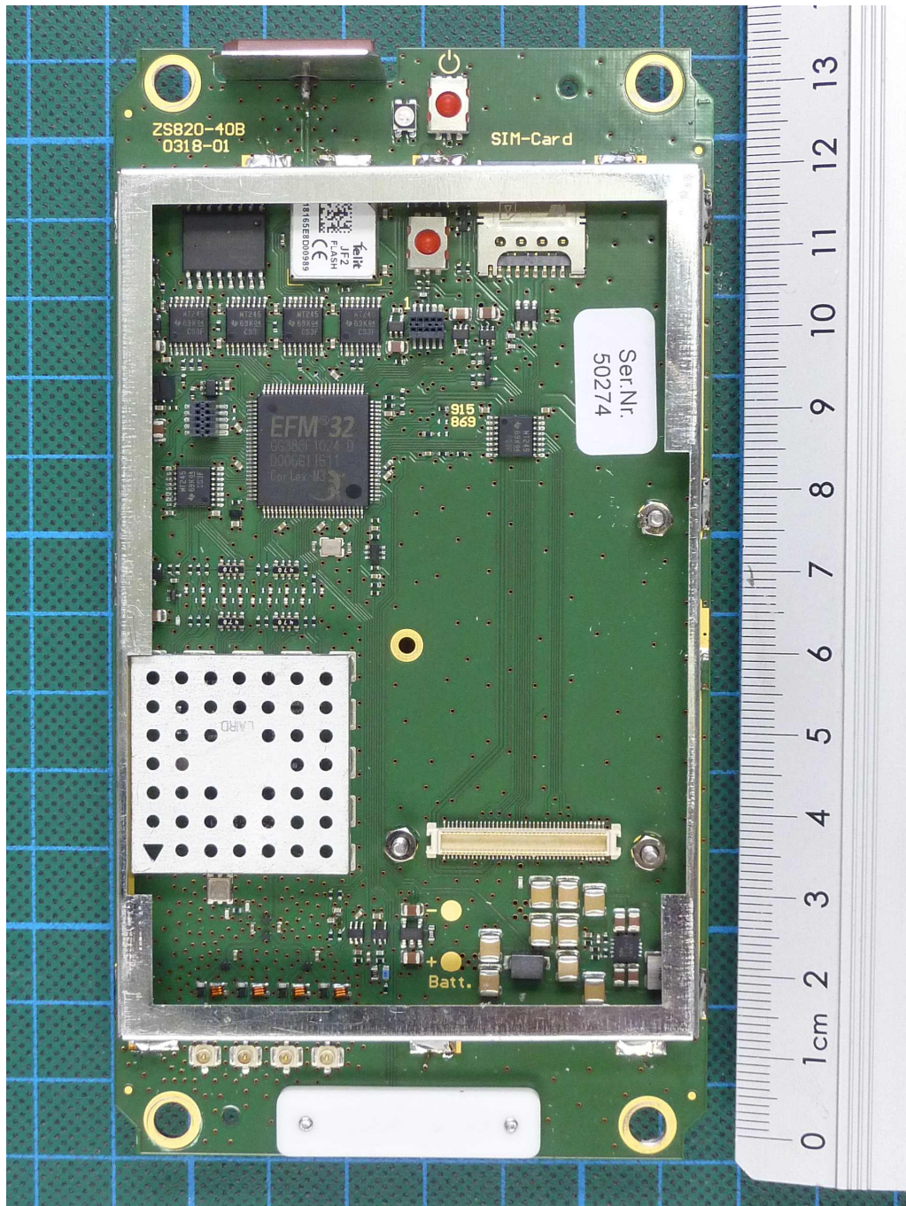
ZONESCAN 820 Alpha V2, main PCB, top view
