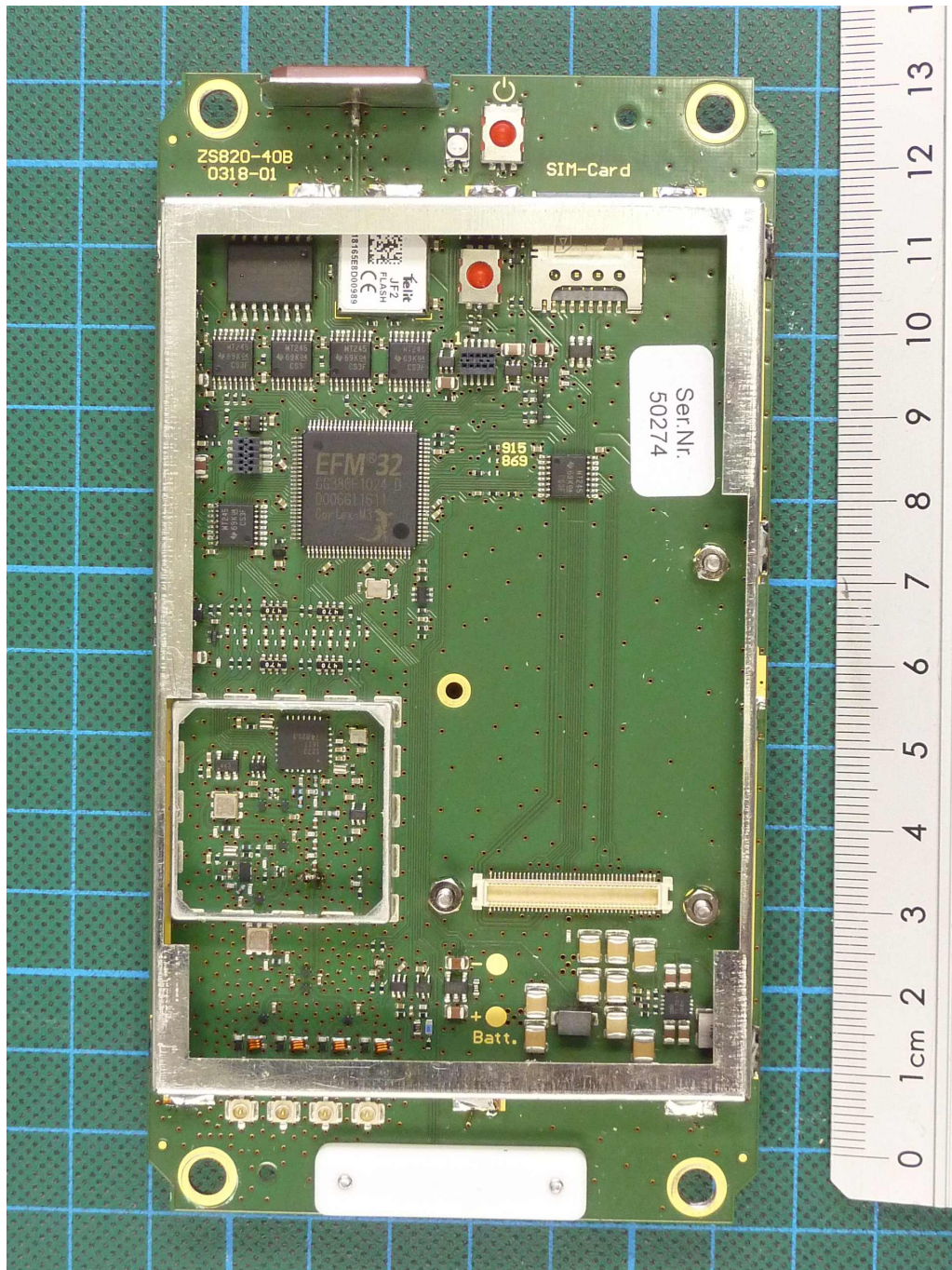
ZONESCAN 820 Alpha V2, main PCB, top view, shielding removed
