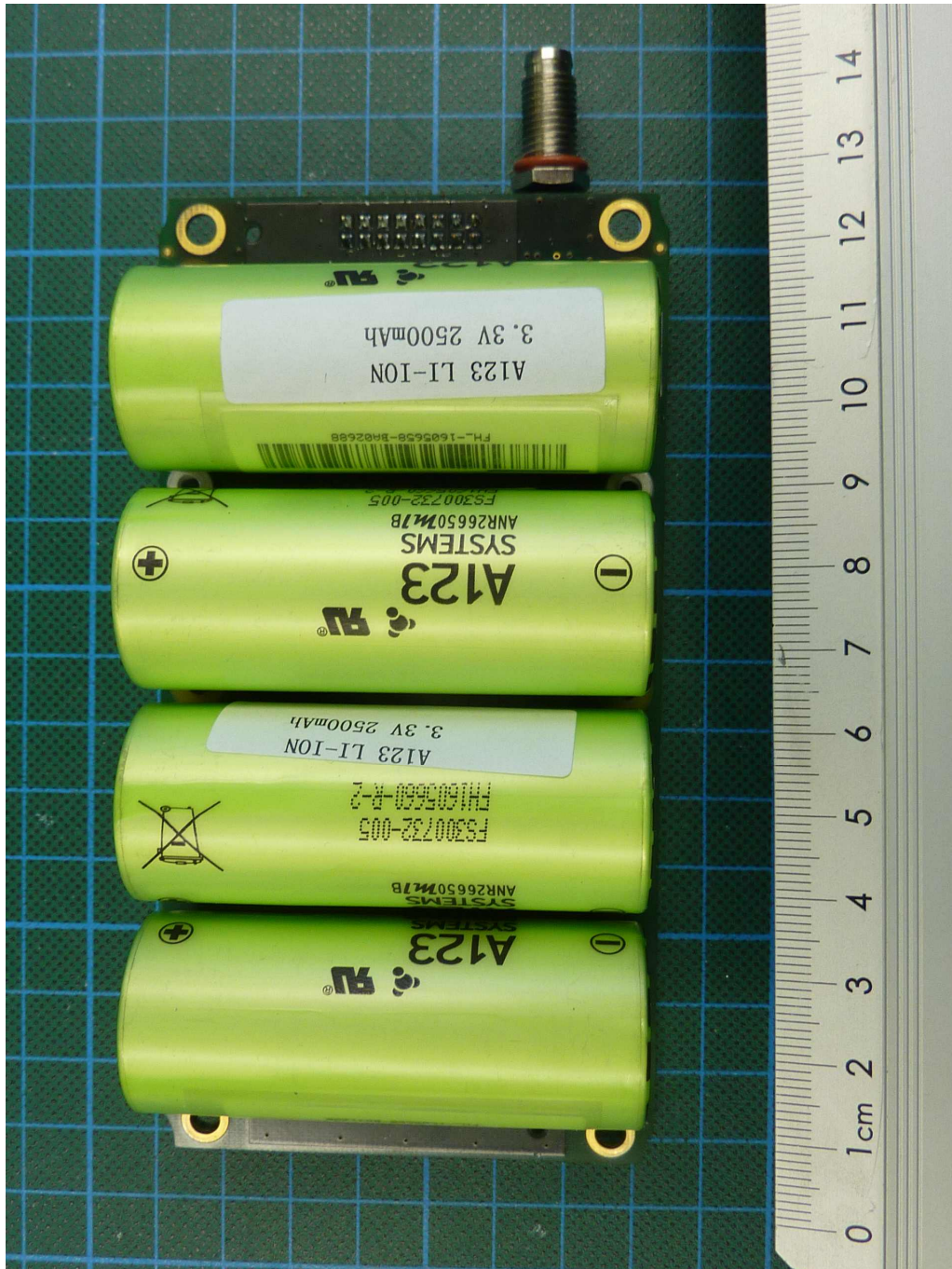
ZONESCAN 820 Alpha V2, battery PCB, bottom view (battery holder removed)
