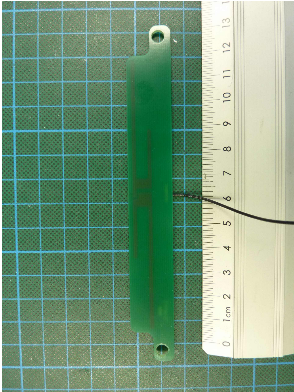
ZONESCAN 820 Alpha V2, FHSS antenna, bottom view
