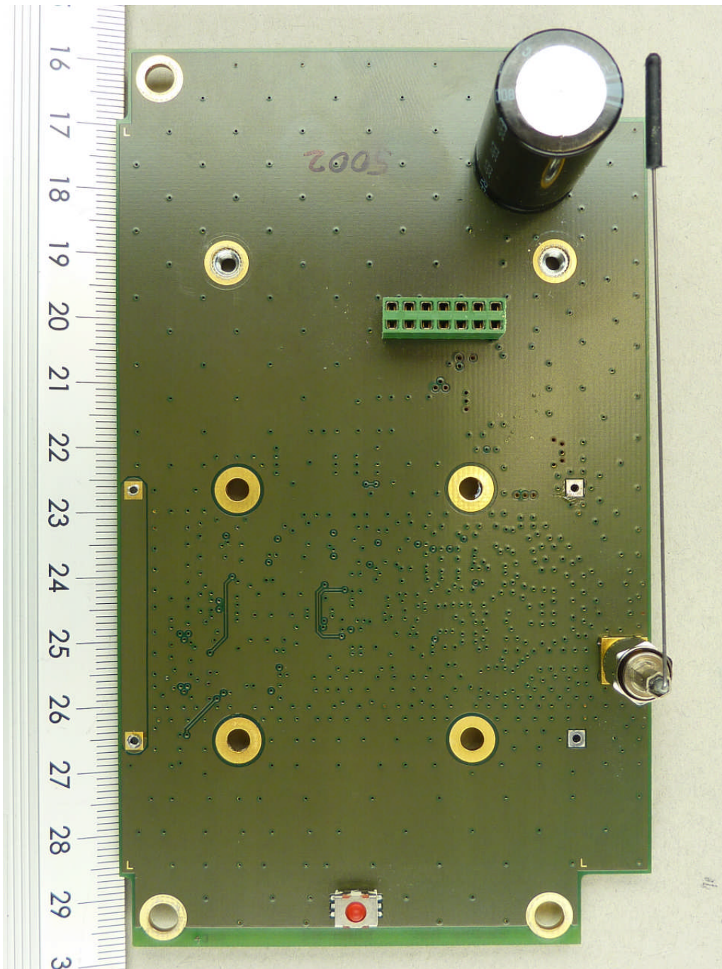
113573_i.JPG: ZONESCAN 820 ALPHA, PCB, top view (battery holder and GPRS module removed)
