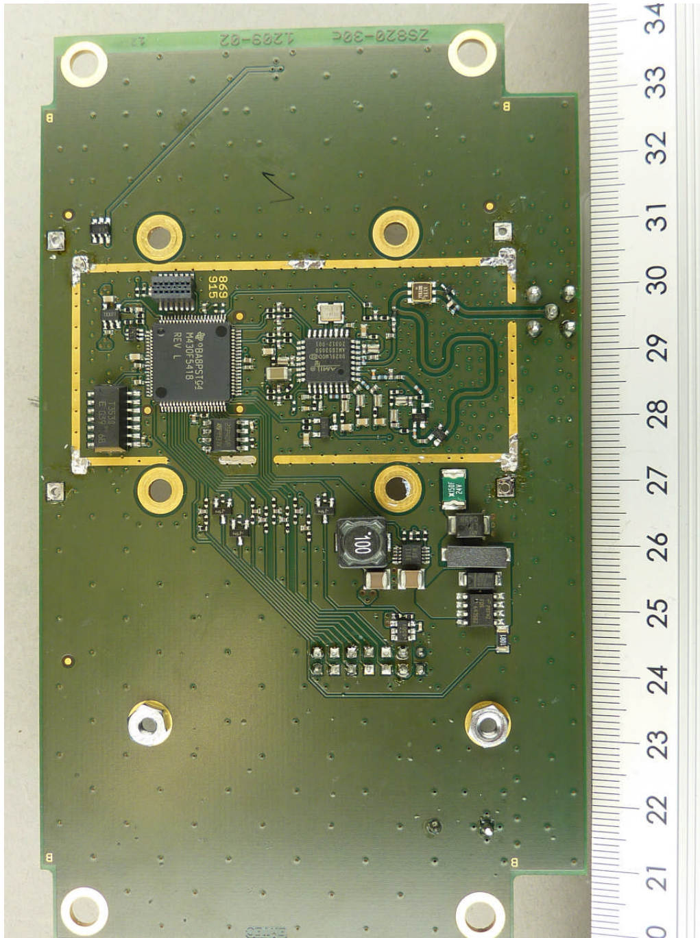
113573_k.JPG: ZONESCAN 820 ALPHA, PCB, bottom view (shielding removed)
