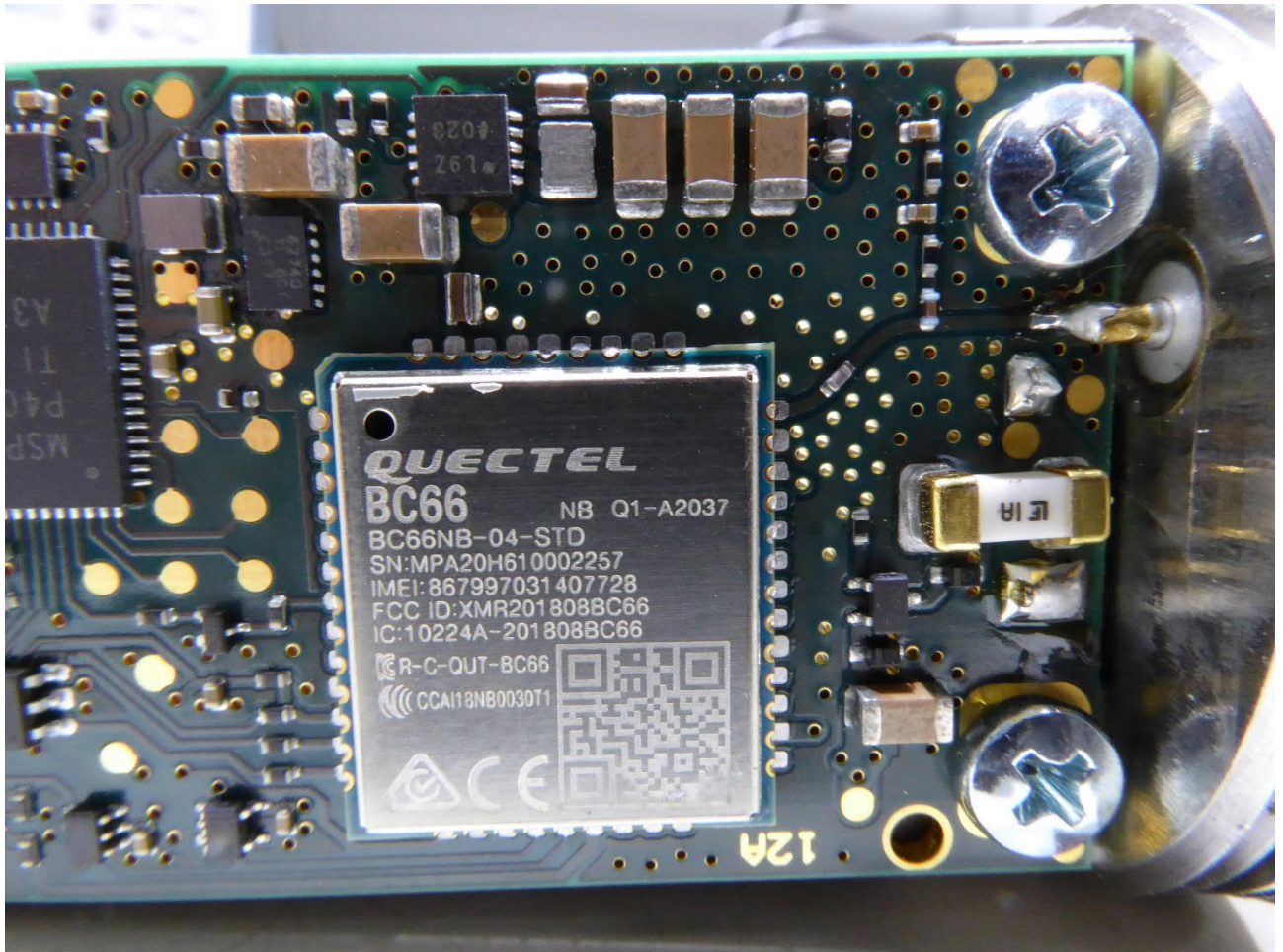
EUT, detail view (FCC / IC label removed)
