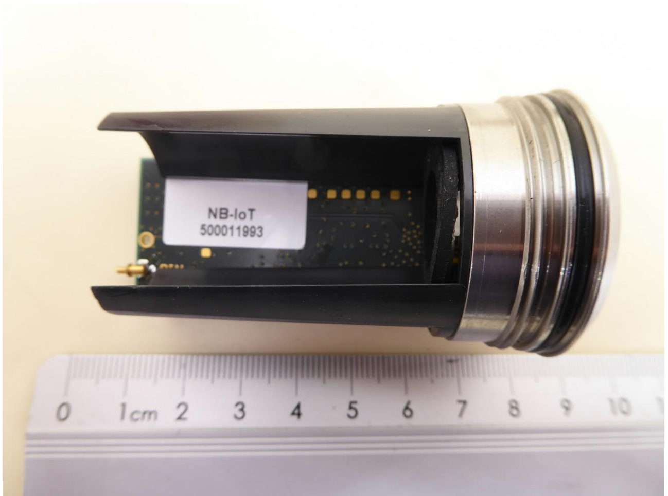
PCB of IoT Leak Logger (host device), bottom view
