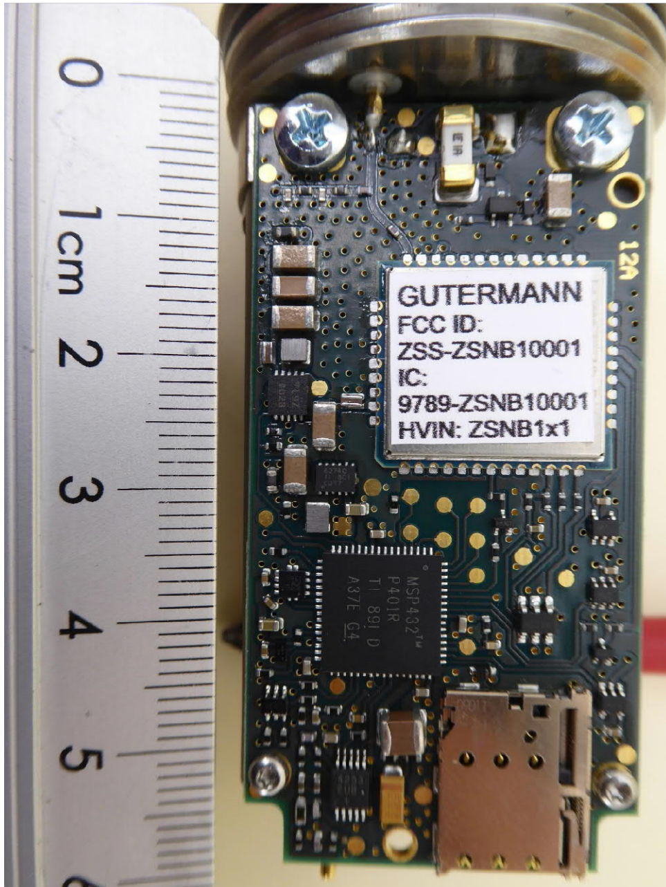
EUT, detail view, labeled (not finalized)
