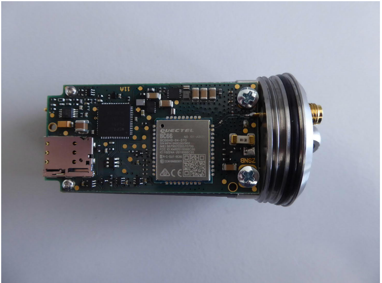
EUT on PCB of IoT Leak Logger (host device), top view
