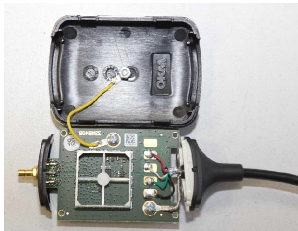
Programming JIG Internal Top view (provided by applicant)
