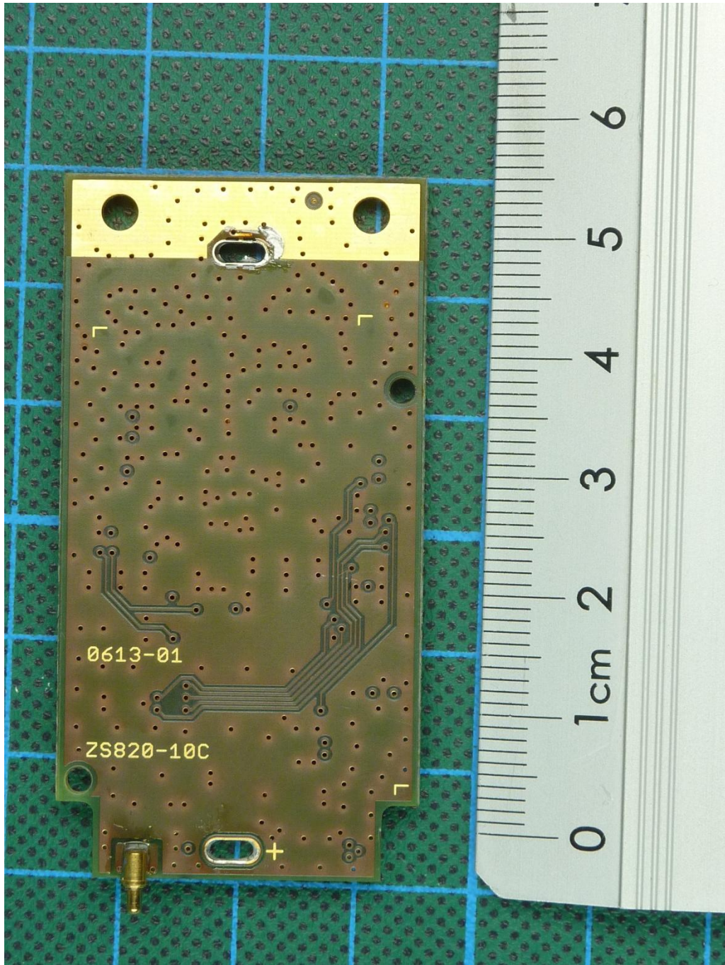
153494_E_U_11.JPG: EASYSCAN SENSOR, PCB, bottom view
