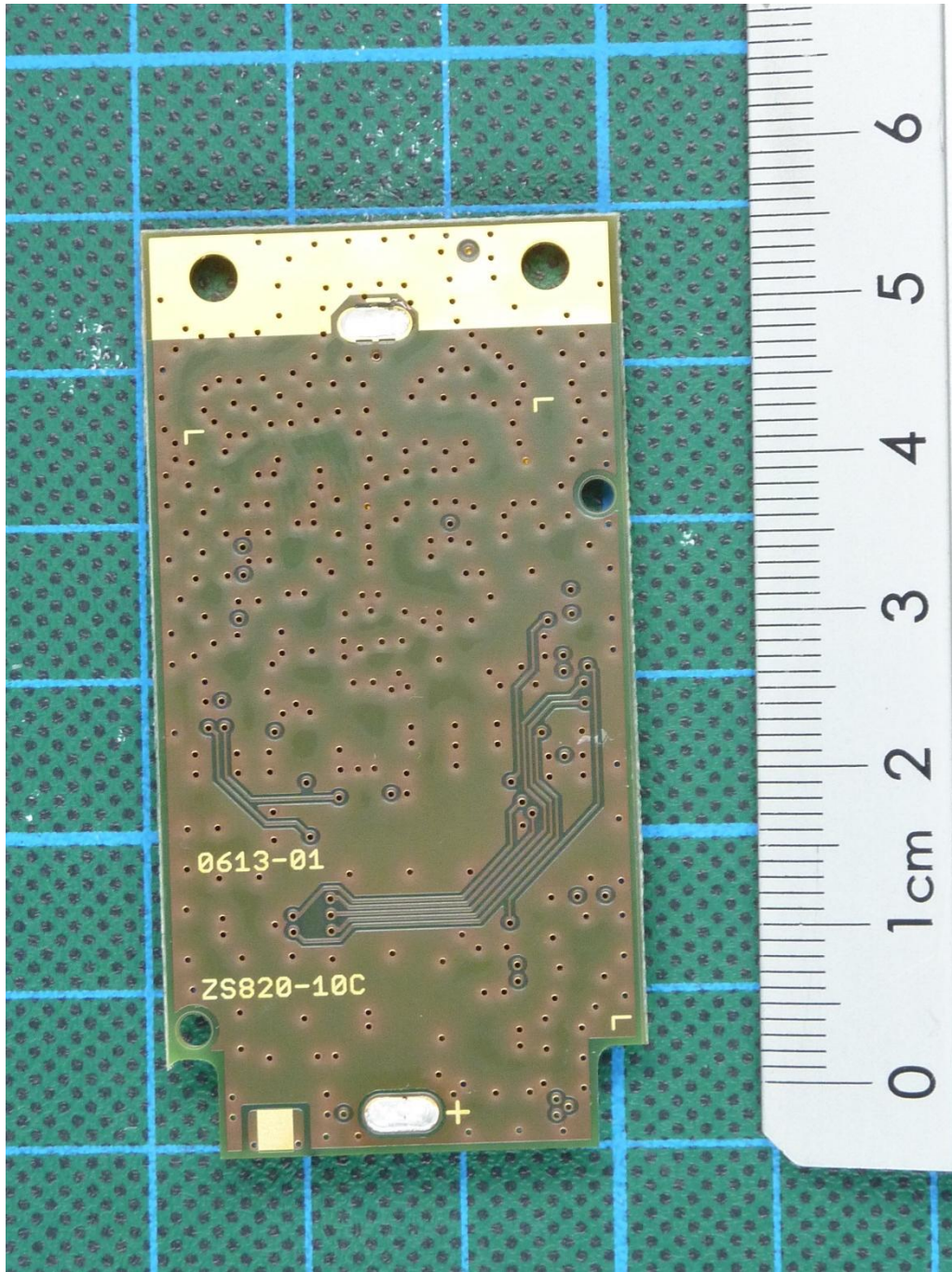
153494_R_U_11.JPG: ZONESCAN 820 Repeater, PCB, bottom view
