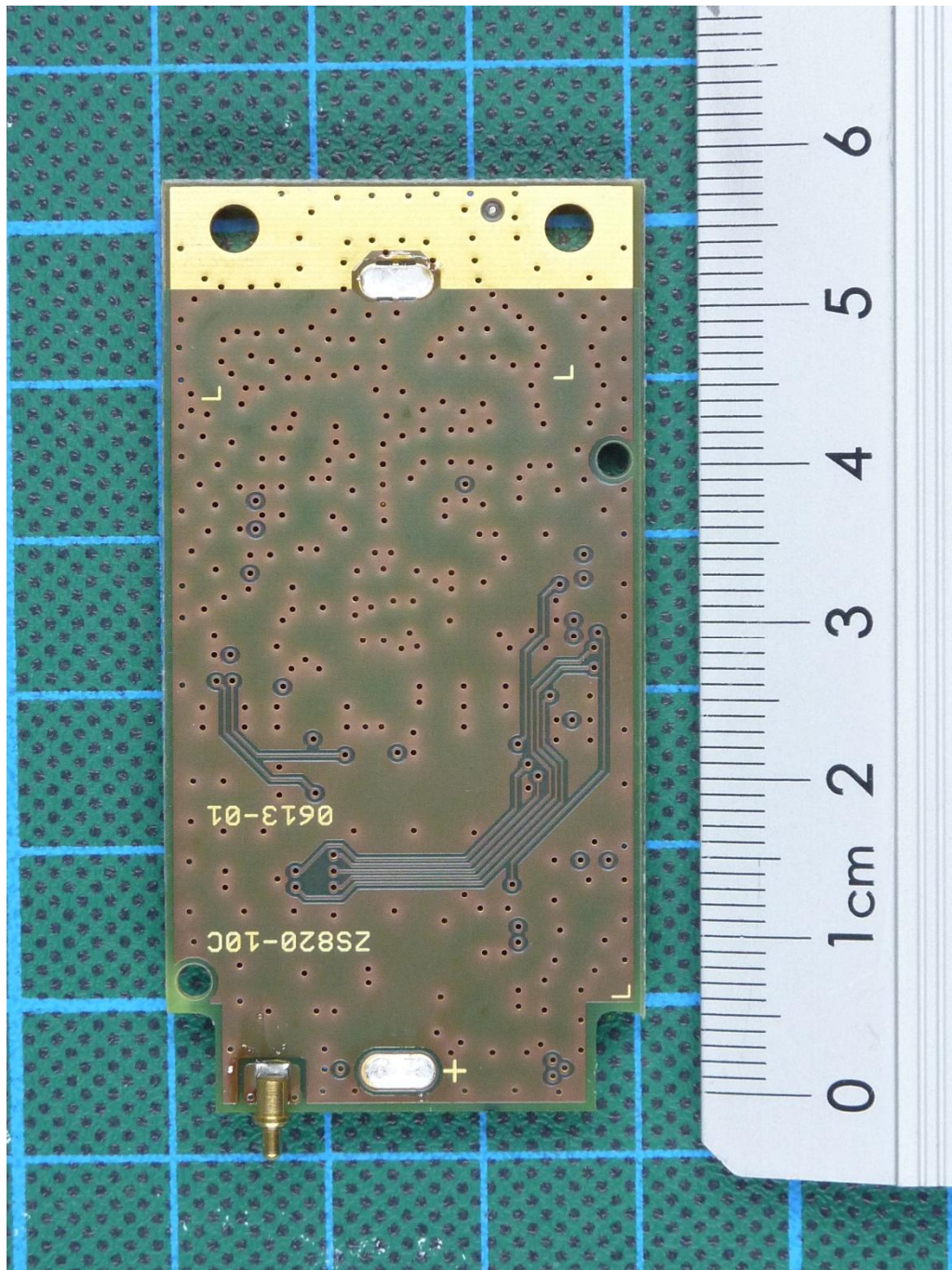
153494_X_U_8.JPG: ZONESCAN 820 Logger with external antenna port, PCB, bottom view
