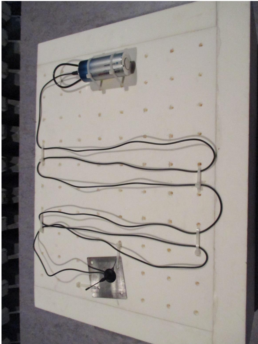
153494_X_U_A.JPG: ZONSCAN 820 Logger with integrated antenna, test setup fully anechoic chamber
