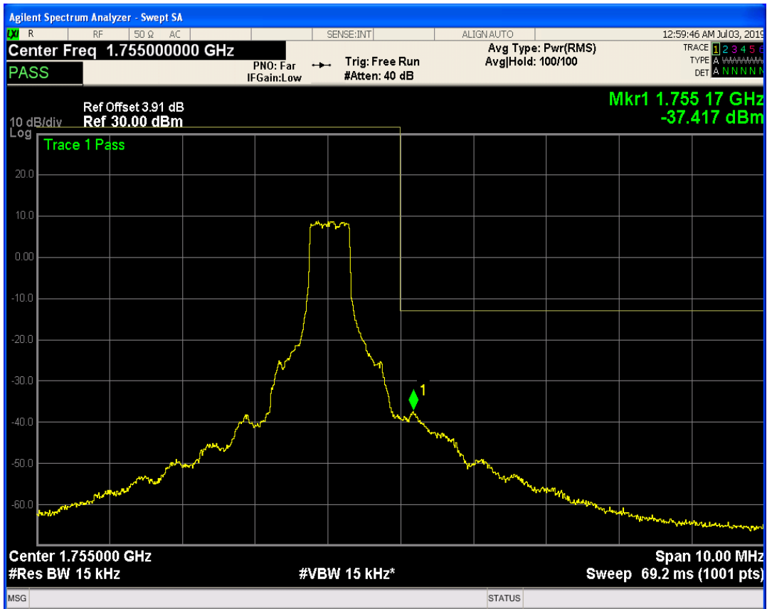
LTE Band4 QPSK BW=1.4MHz Channel=20393 RB Size=3 Position=#0
