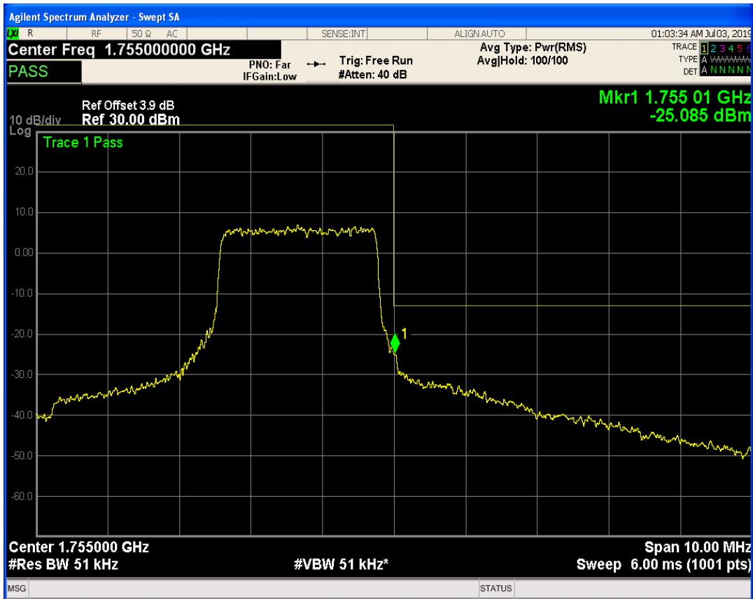
LTE Band4 QAM16 BW=5MHz Channel=20375 RB Size=12 Position=#Max
