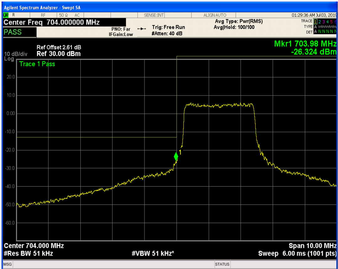
LTE Band17 QAM16 BW=5MHz Channel=23755 RB Size=12 Position=#0
