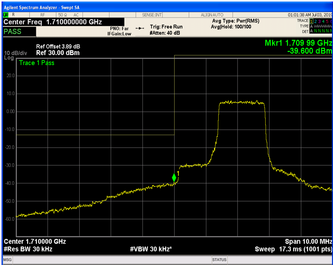
LTE Band4 QAM16 BW=3MHz Channel=19965 RB Size=8 Position=#Max
