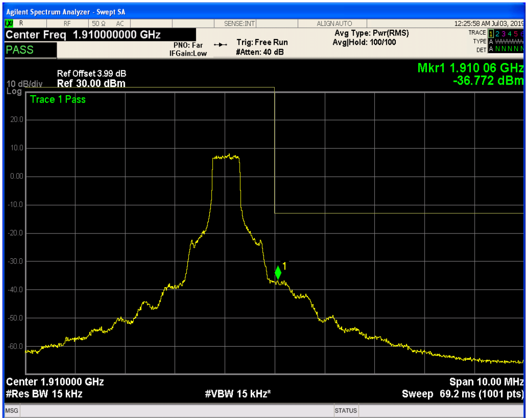
LTE Band2 QPSK BW=1.4MHz Channel=19193 RB Size=3 Position=#0
