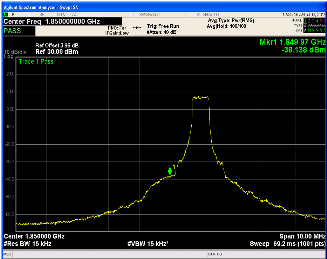
LTE Band2 QAM16 BW=15MHz Channel=18675 RB Size=36 Position=#Max
