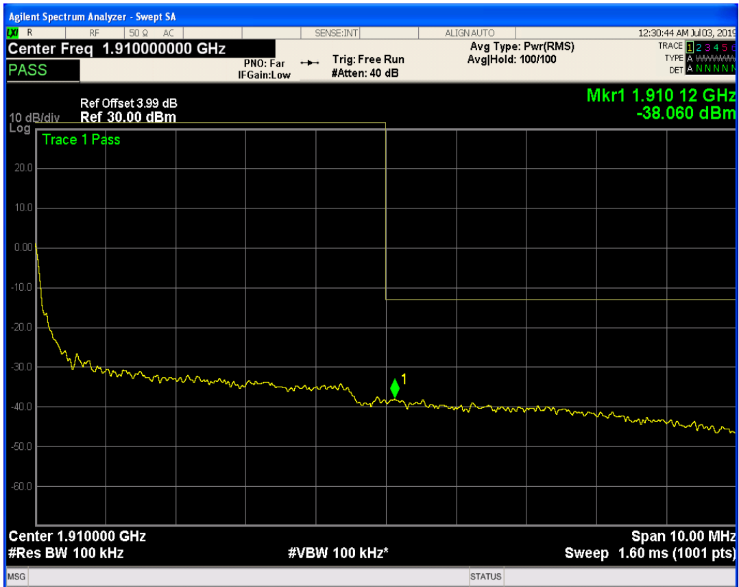
LTE Band2 QAM16 BW=10MHz Channel=19150 RB Size=25 Position=#0
