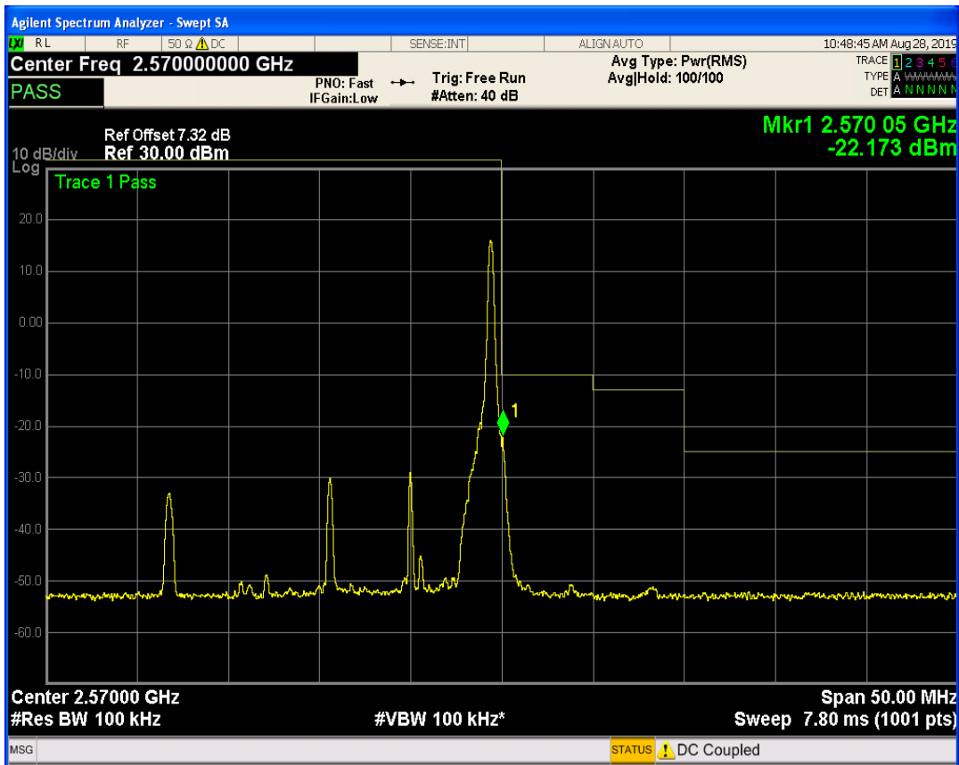
LTE Band7 QPSK BW=10MHz Channel=21400 RB Size=25 Position=#0
