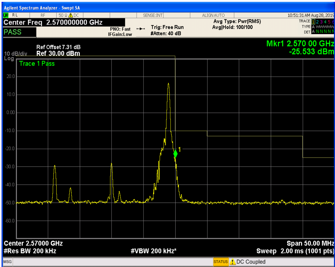
LTE Band7 QAM16 BW=20MHz Channel=21350 RB Size=50 Position=#Max
