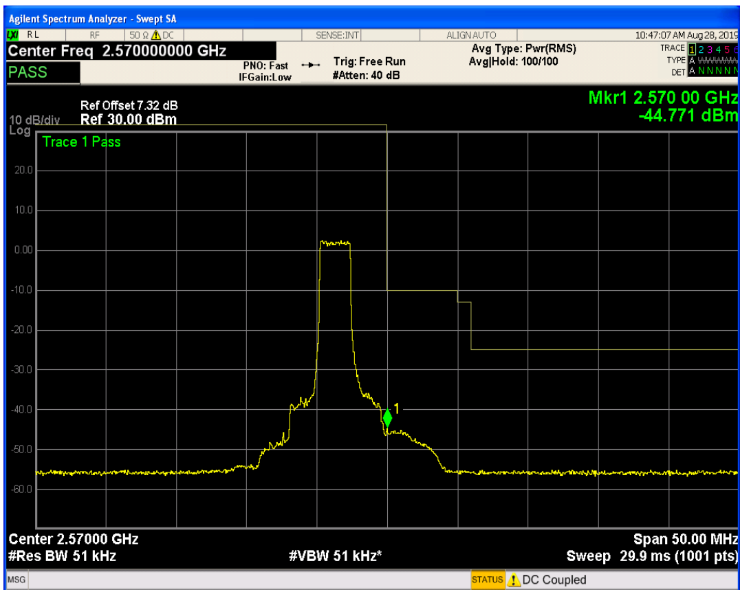
LTE Band7 QPSK BW=5MHz Channel=21425 RB Size=12 Position=#Max
