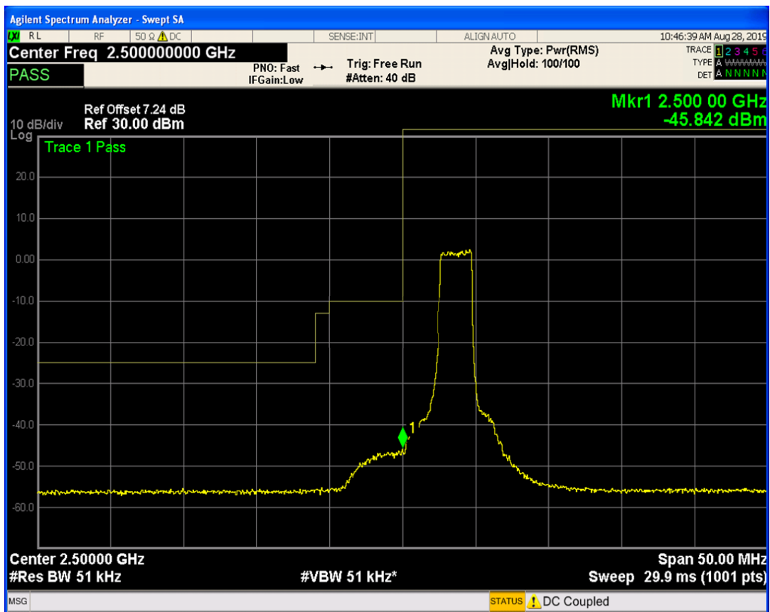
LTE Band7 QAM16 BW=5MHz Channel=20775 RB Size=12 Position=#Max
