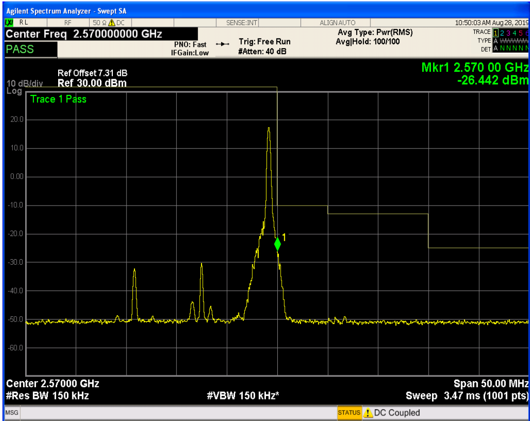
LTE Band7 QPSK BW=15MHz Channel=21375 RB Size=36 Position=#0
