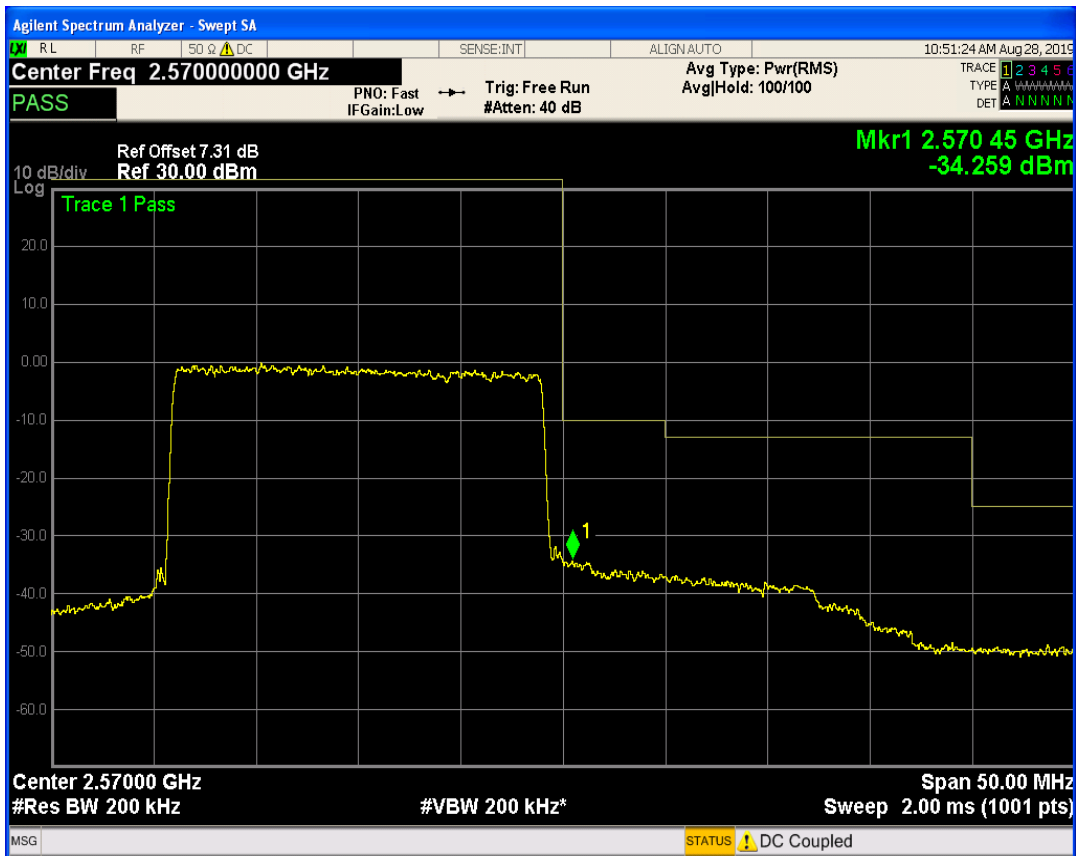
LTE Band7 QPSK BW=20MHz Channel=21350 RB Size=50 Position=#0
