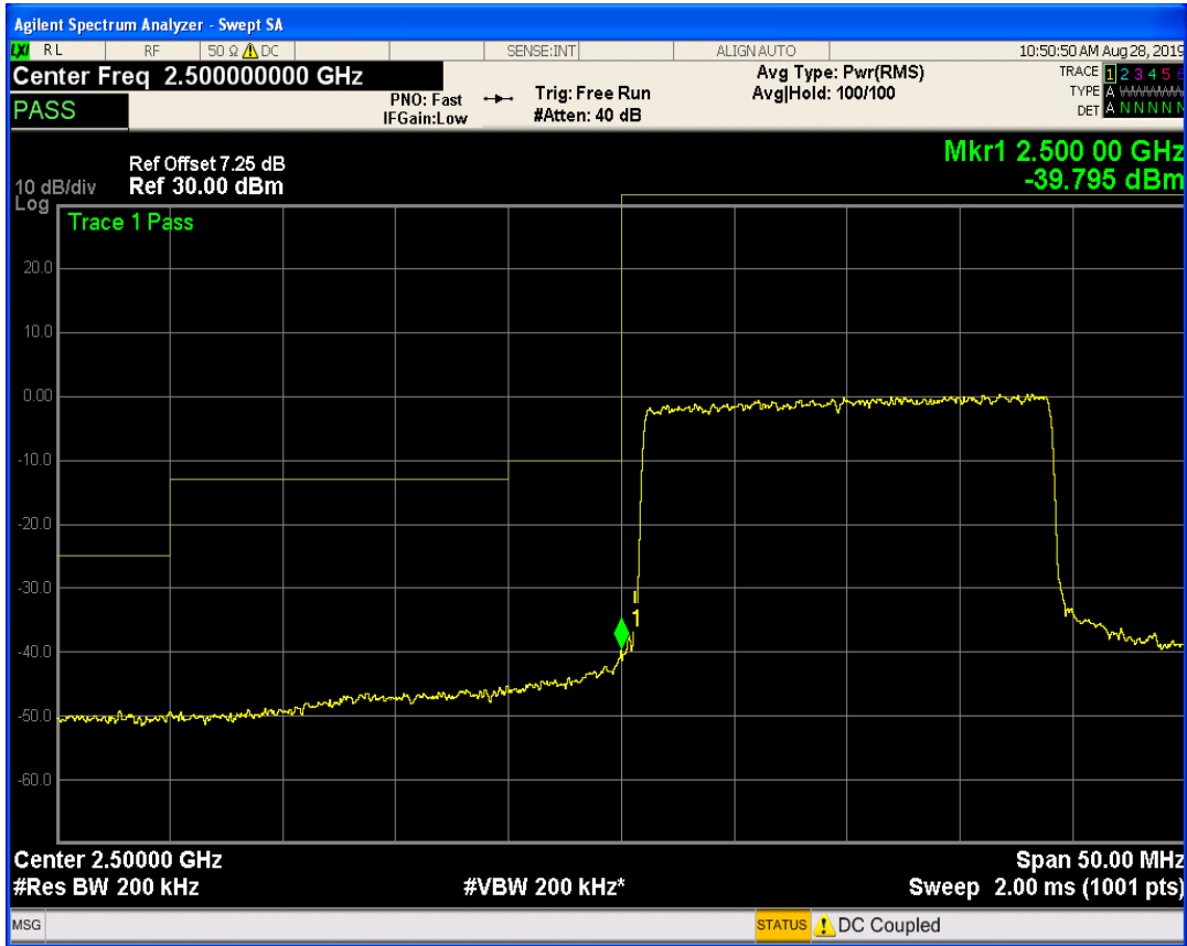
LTE Band7 QPSK BW=20MHz Channel=20850 RB Size=50 Position=#0
