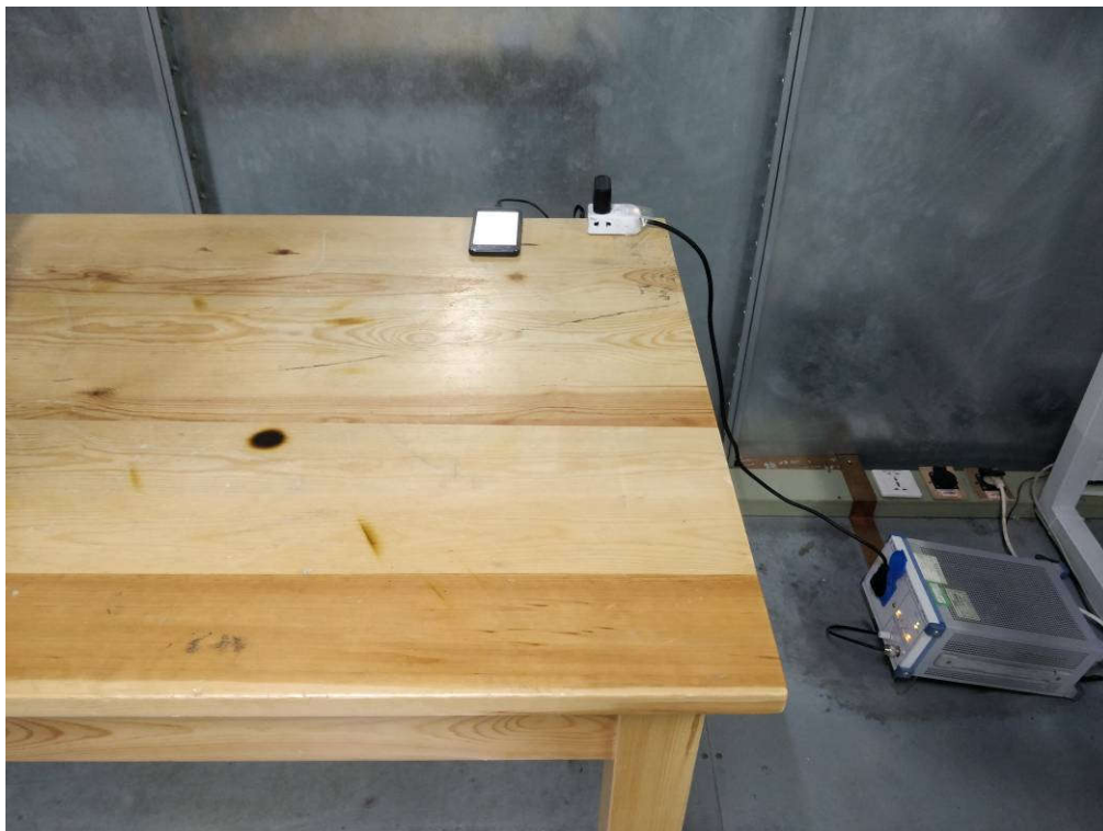
Conducted Emission-AC charging mode
