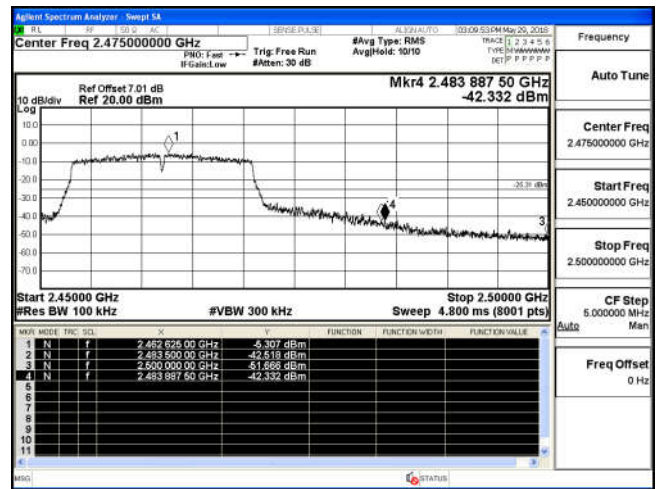
Channel 11 / 2462 MHz
