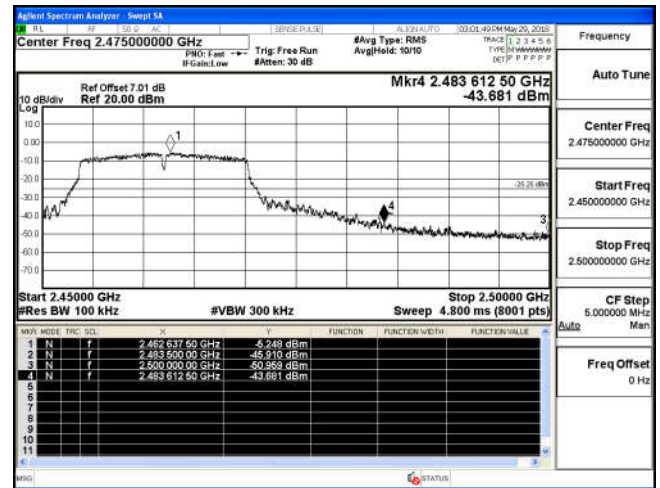
Channel 11 / 2462 MHz
