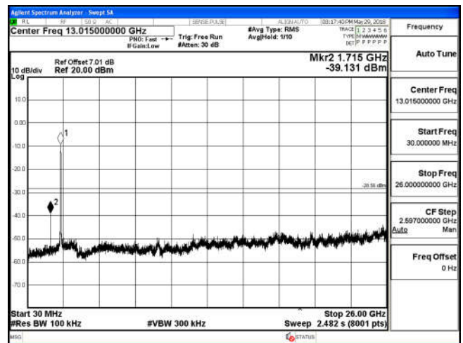
30 MHz – 26 GHz
