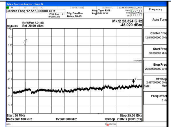
30 MHz – 25 GHz
