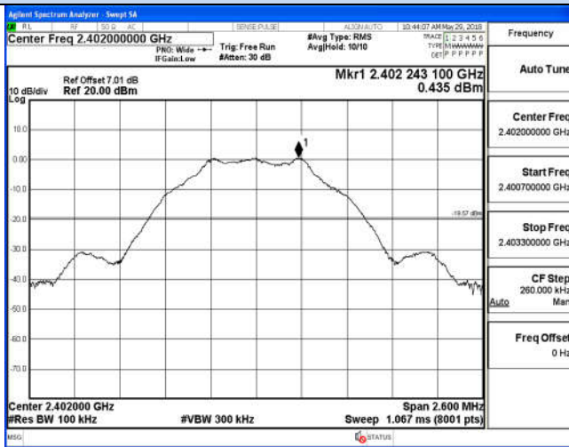
2400.7 MHz – 2403.3 MHz
