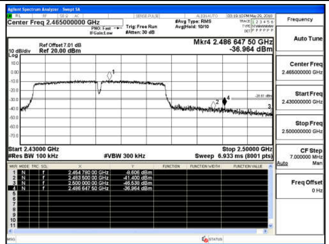
Channel 9 / 2452 MHz
