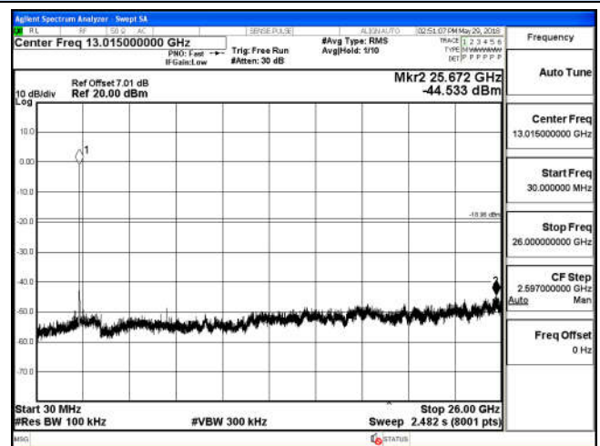
30 MHz – 26 GHz
