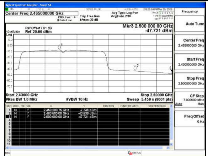
Channel 9 / 2452 MHz – Average
