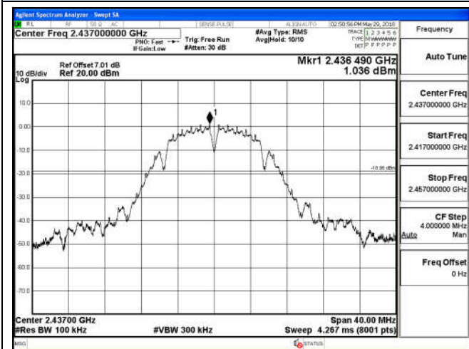
2417 MHz – 2457 MHz
