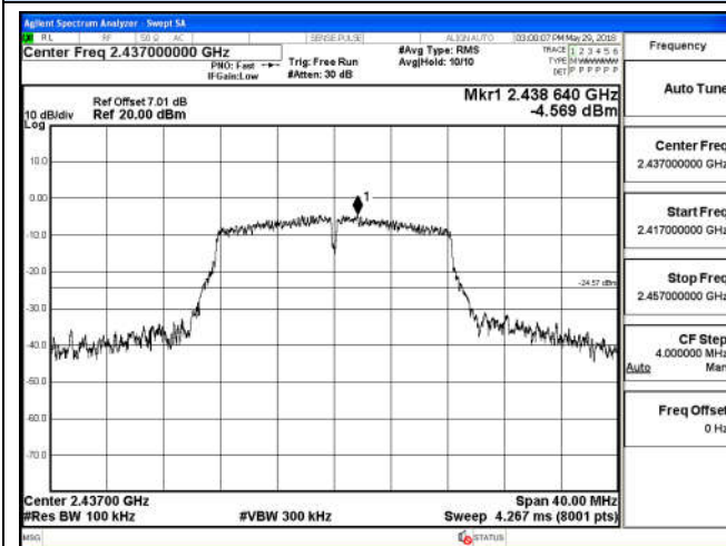
2417 MHz – 2457 MHz
