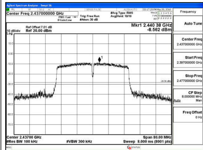
2397 MHz – 2477 MHz
