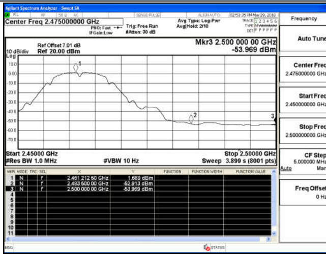
Channel 11 / 2462 MHz – Average IEEE 802.11n HT20
