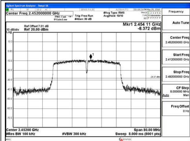
2412 MHz – 2492 MHz
