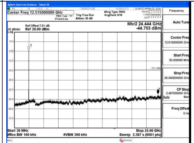
30 MHz – 25 GHz
