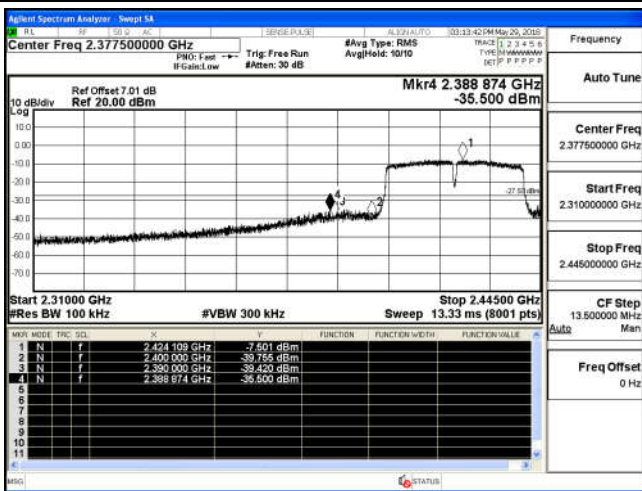
Channel 3 / 2422 MHz
