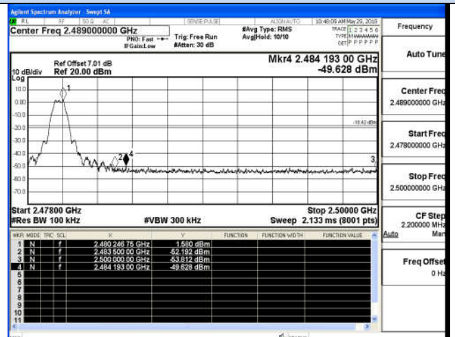
Channel 39 / 2480 MHz
