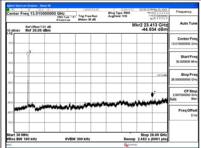
30 MHz – 26 GHz
