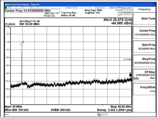
30 MHz – 26 GHz
