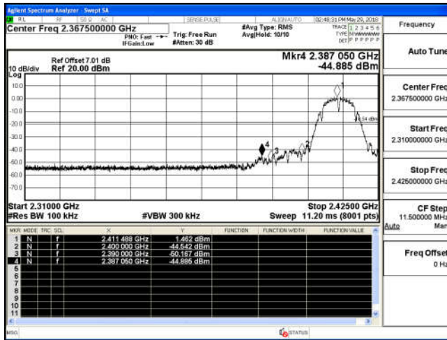
Channel 1 / 2412 MHz
