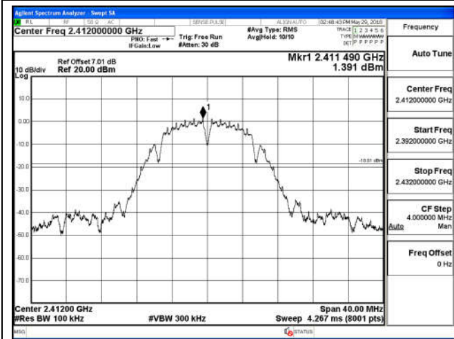
2392 MHz – 2432 MHz
