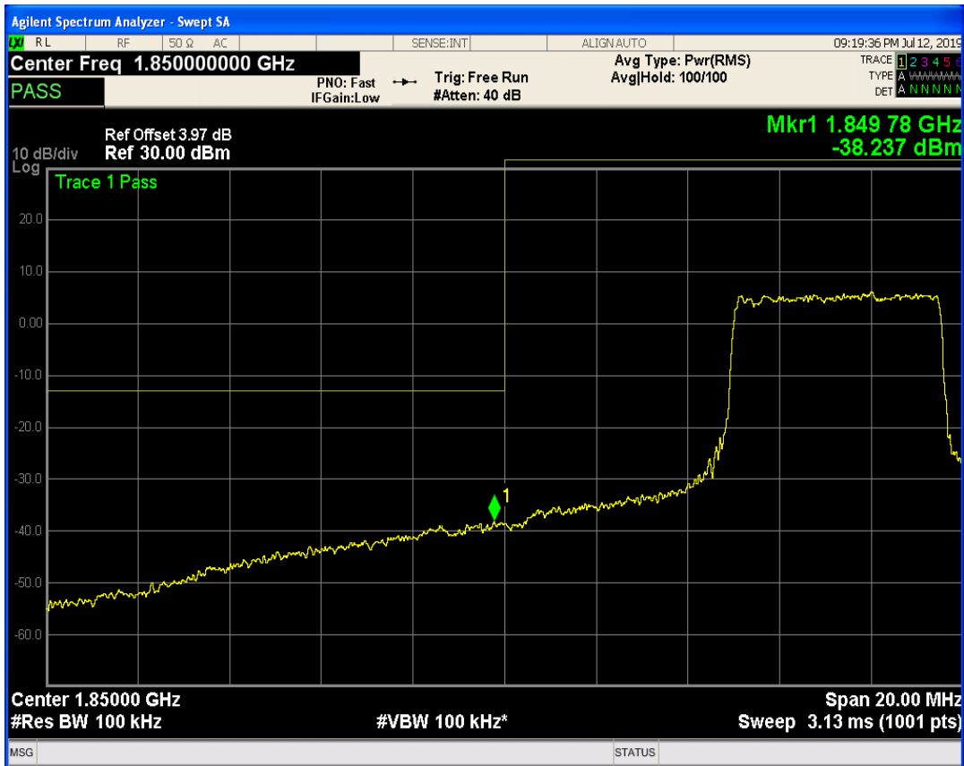
LTE Band2 QAM16 BW=10MHz Channel=18650 RB Size=25 Position=#Max
