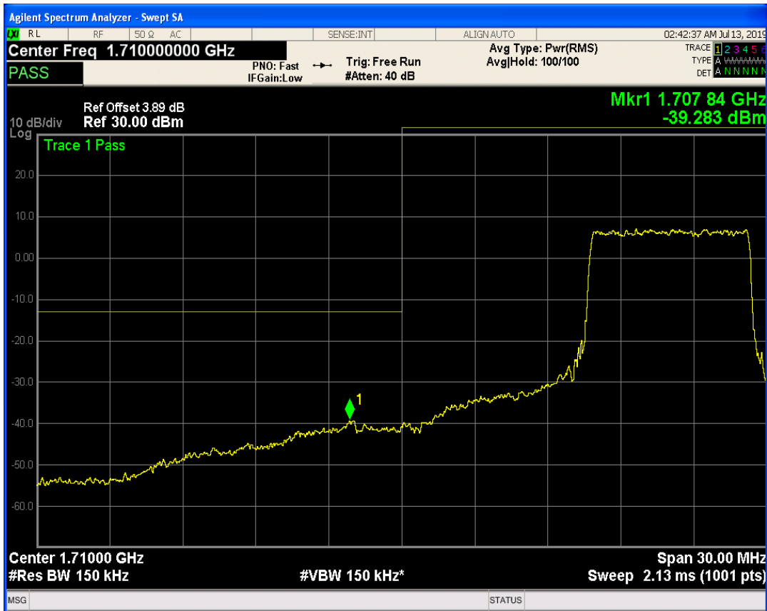
LTE Band4 QPSK BW=15MHz Channel=20025 RB Size=36 Position=#Max
