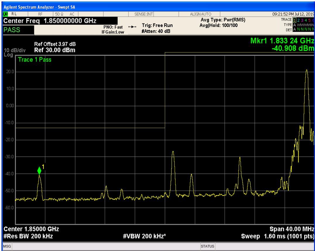
LTE Band2 QAM16 BW=20MHz Channel=18700 RB Size=50 Position=#0
