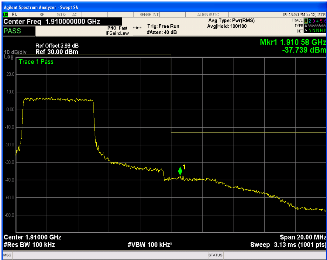
LTE Band2 QPSK BW=10MHz Channel=19150 RB Size=25 Position=#Max
