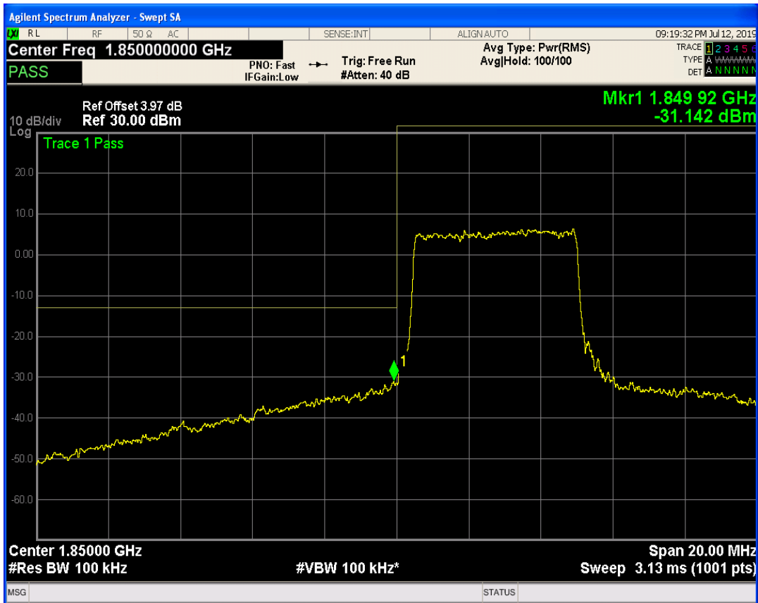
LTE Band2 QAM16 BW=10MHz Channel=18650 RB Size=25 Position=#0
