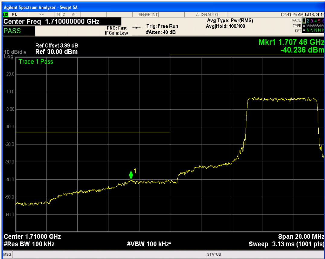
LTE Band4 QPSK BW=10MHz Channel=20000 RB Size=25 Position=#Max
