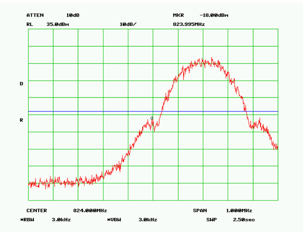
Lower Band Edge Plot – EGPRS850, Channel 128, Low Channel
