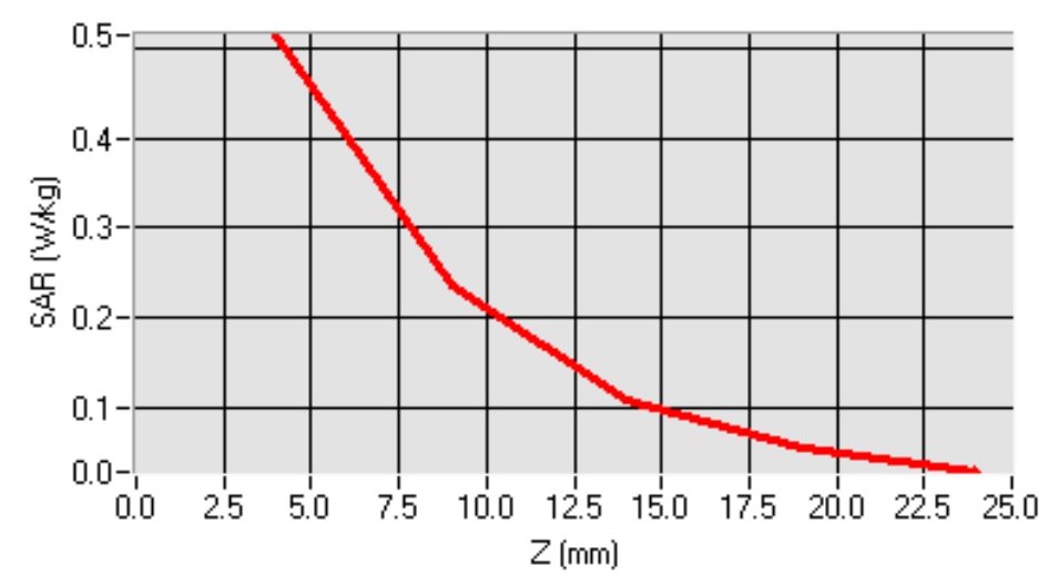
SAR, Z Axis Scan (X = -7, Y = -22)
