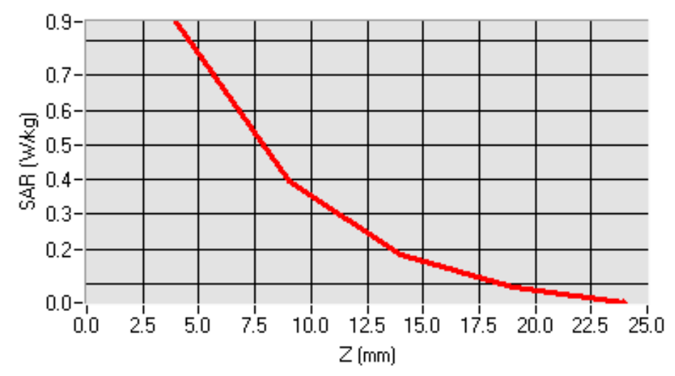
SAR, Z Axis Scan (X = -3, Y = -8)
