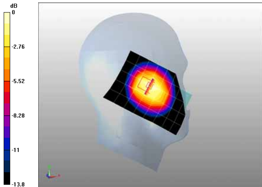
0 dB = 1.26mW/g
