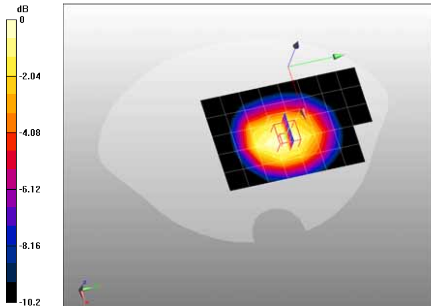
0 dB = 1.02mW/g
