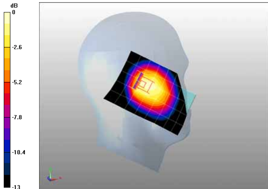
0 dB = 0.835mW/g
