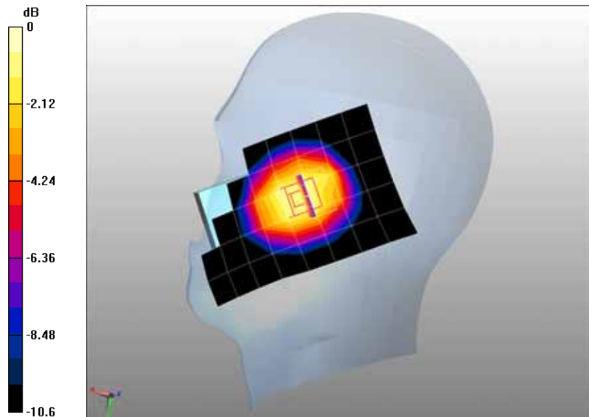
0 dB = 1.26mW/g
