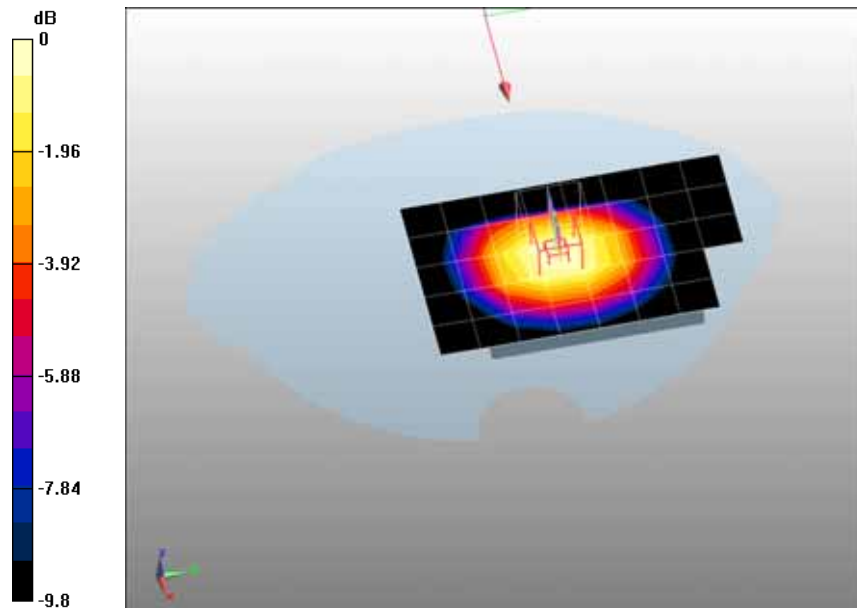
0 dB = 0.677mW/g
