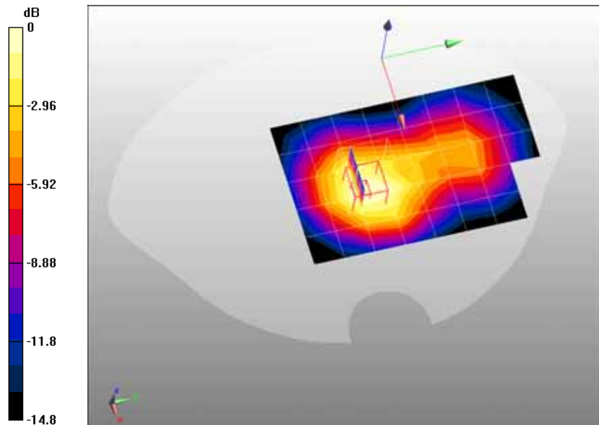
0 dB = 0.198mW/g
