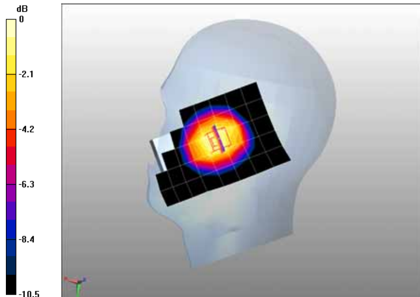
0 dB = 1.27mW/g
