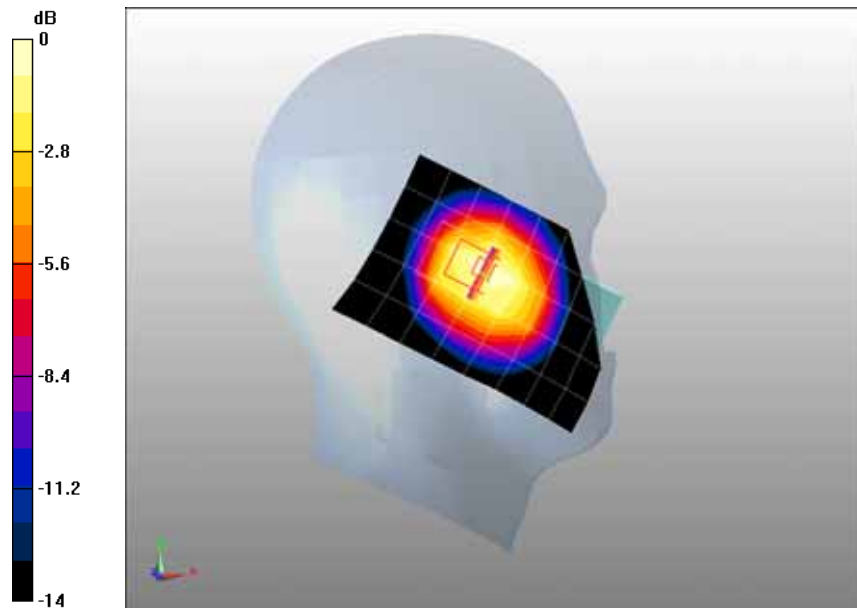
0 dB = 1.25mW/g
