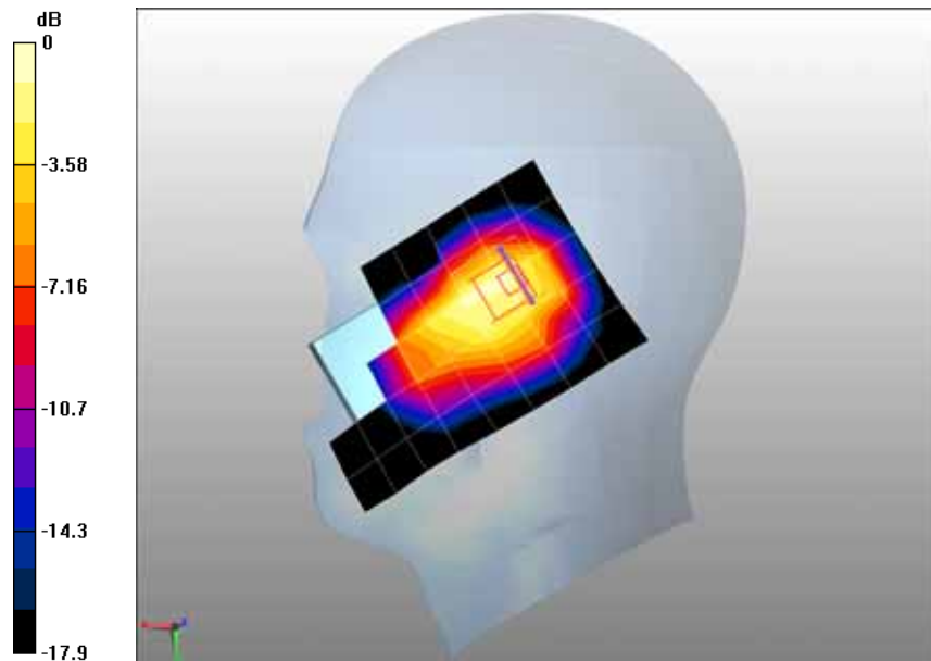
0 dB = 0.856mW/g
