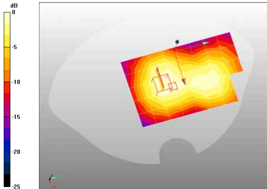
0 dB = 0.121mW/g
