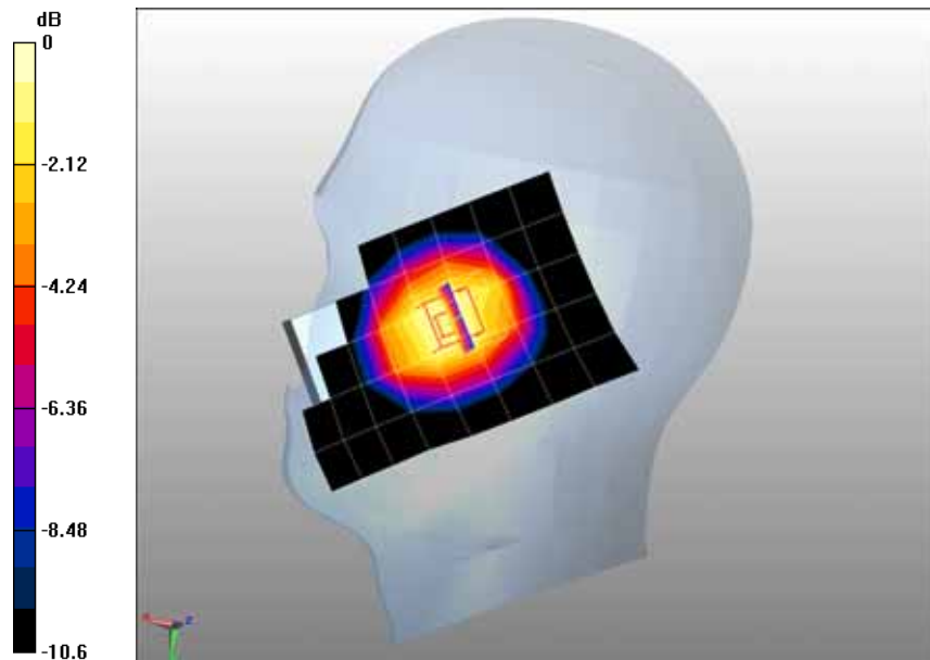
0 dB = 1.2mW/g
