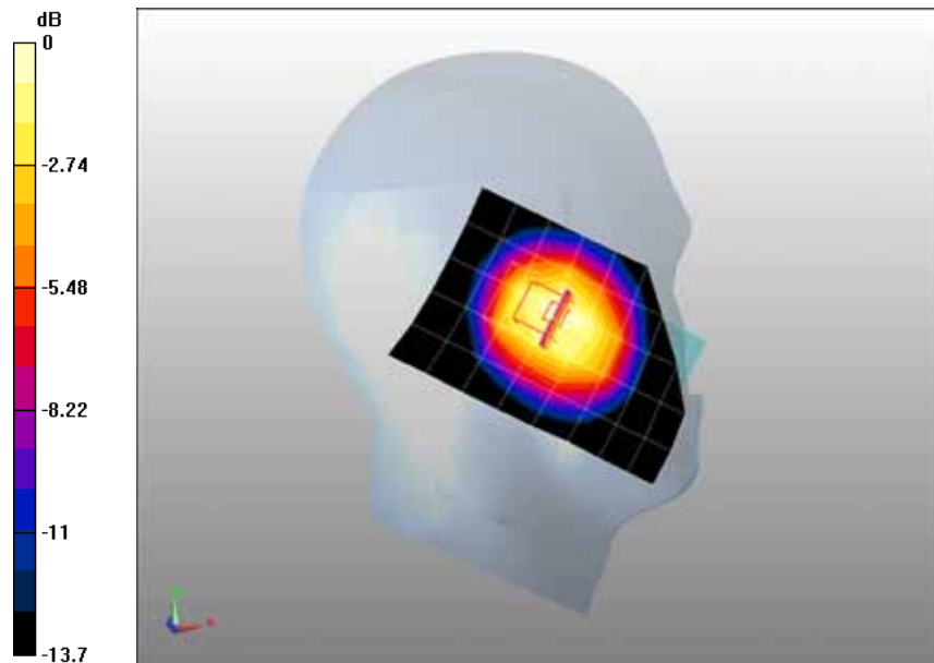
0 dB = 1.13mW/g
