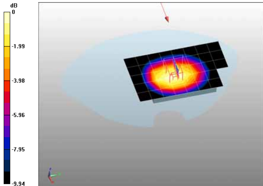
0 dB = 0.817mW/g
