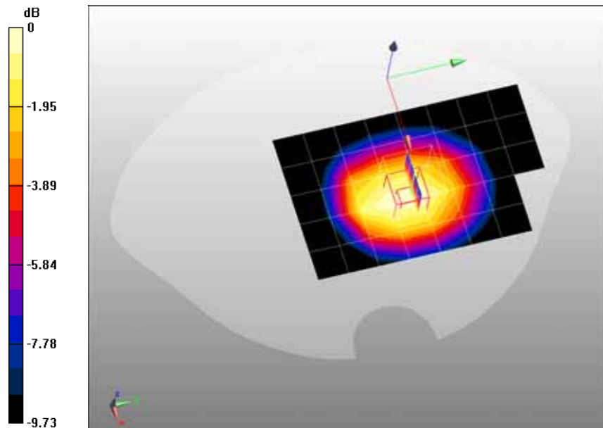
0 dB = 0.863mW/g
