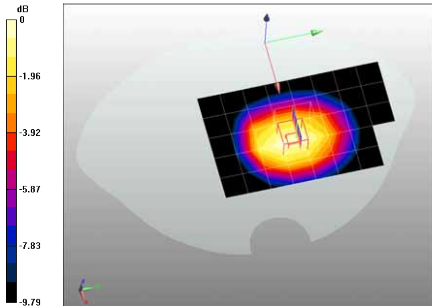
0 dB = 0.488mW/g
