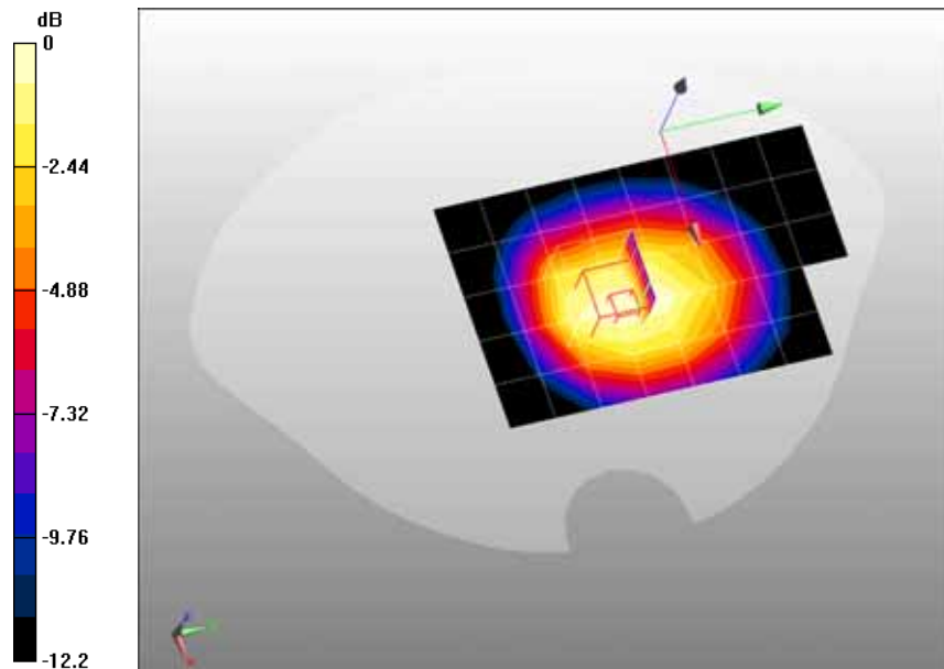
0 dB = 0.910mW/g
