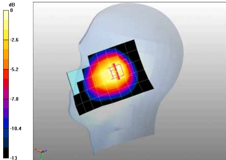
0 dB = 0.885mW/g
