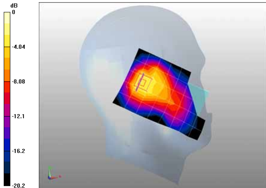
0 dB = 0.591mW/g
