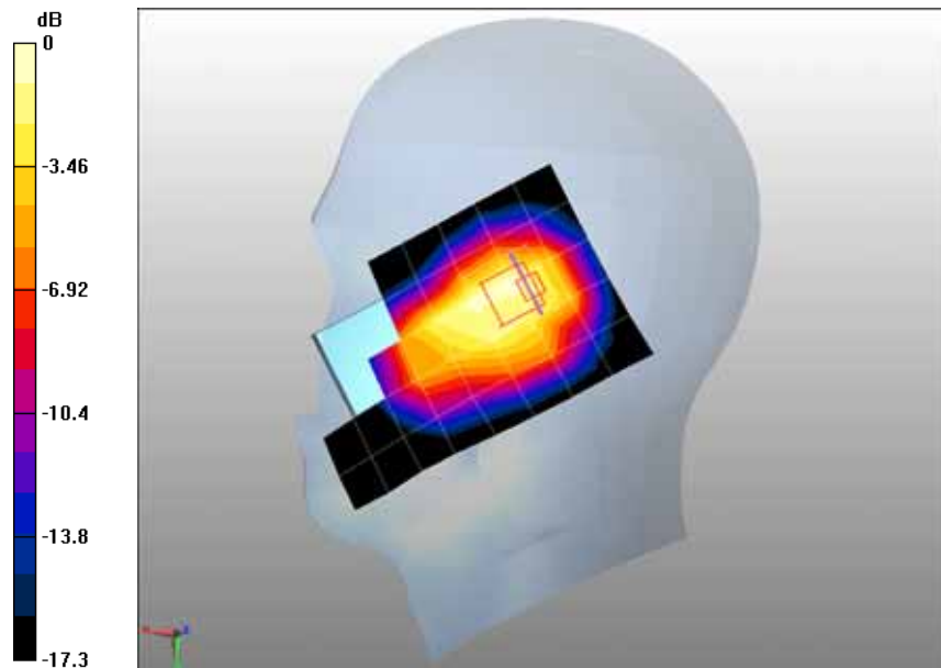
0 dB = 0.780mW/g
