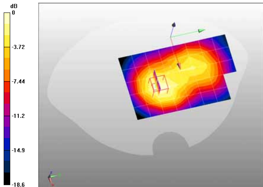
0 dB = 0.157mW/g
