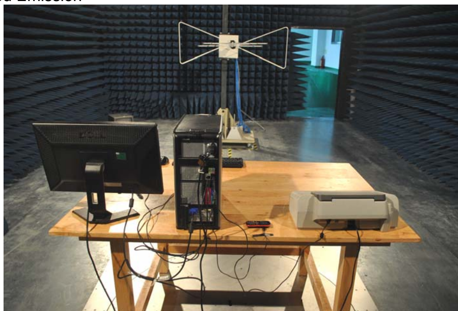
Radiated Emission
