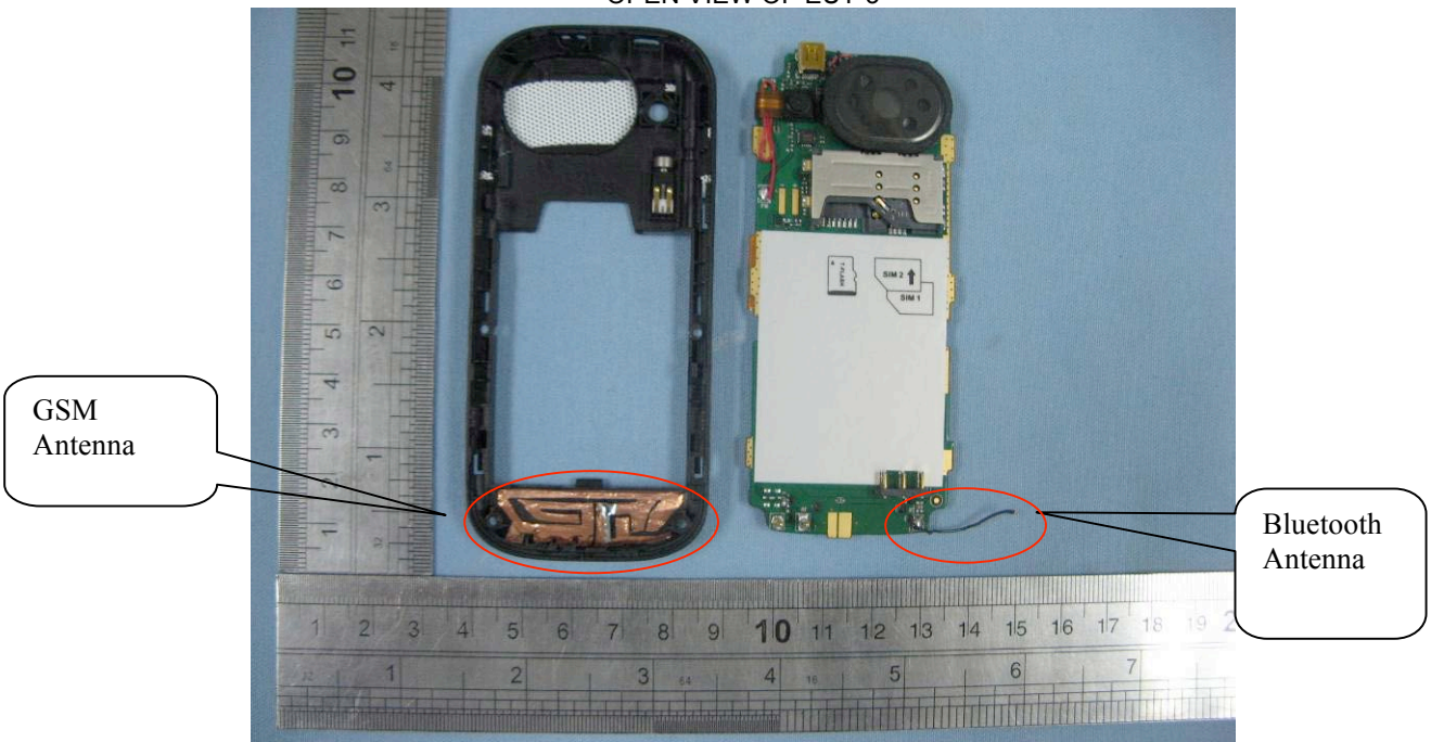
OPEN VIEW OF EUT-3
