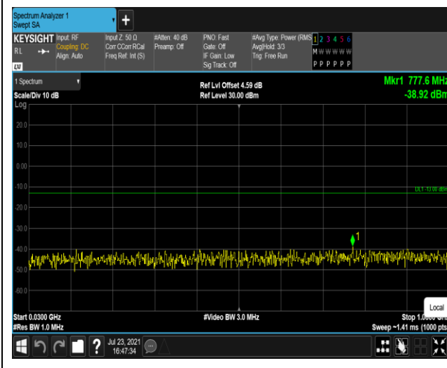
Band2-20MHz-QPSK-19100-1RB#0-Range1:30~1000MHz
