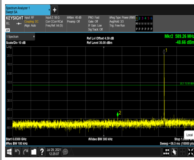
Band5-1.4MHz-16QAM-20525-1RB#0-Range1:30~1000MHz
