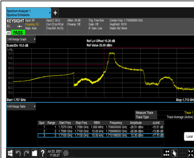
Band4-1.4MHz-QPSK-19957-1RB#0
