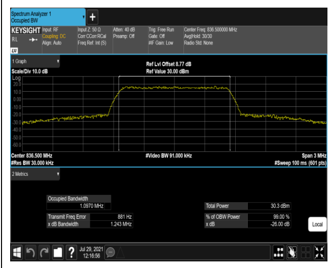
Band5-1.4MHz-16QAM-20525-6RB#0
