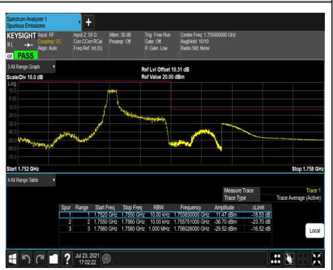
Band4-1.4MHz-16QAM-20393-1RB#0
