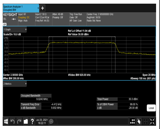
Band7-10MHz-16QAM-21400-50RB#0
