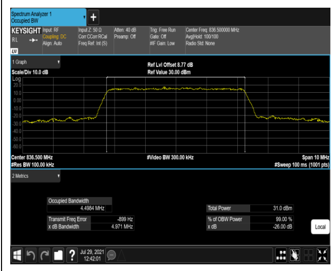
Band5-5MHz-16QAM-20525-25RB#0
