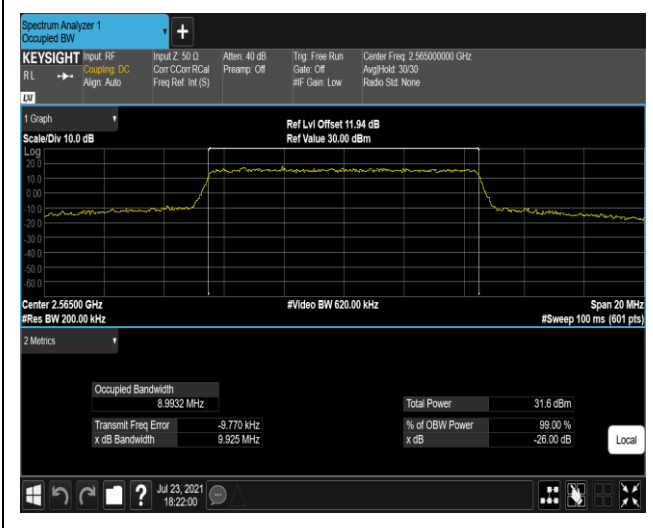
Band7-10MHz-QPSK-21400-50RB#0
