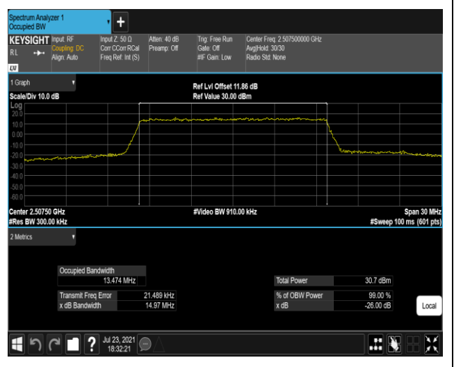
Band7-15MHz-16QAM-20825-75RB#0
