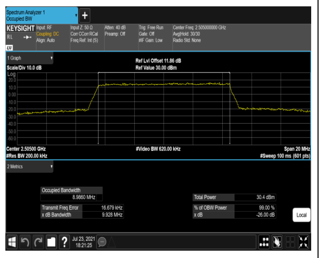
Band7-10MHz-16QAM-20800-50RB#0
