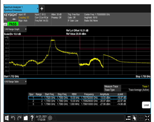
Band4-1.4MHz-QPSK-20393-1RB#0
