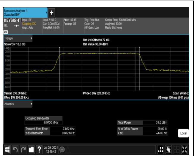
Band5-10MHz-QPSK-20525-50RB#0
