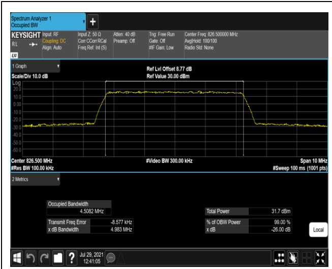
Band5-5MHz-QPSK-20425-25RB#0
