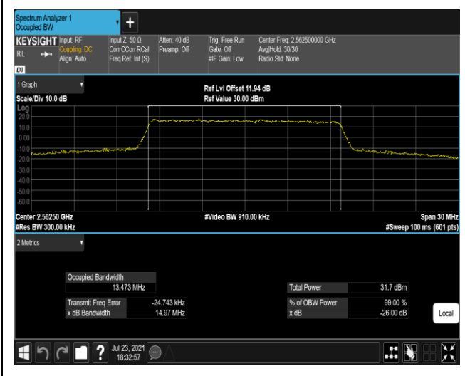
Band7-15MHz-QPSK-21375-75RB#0
