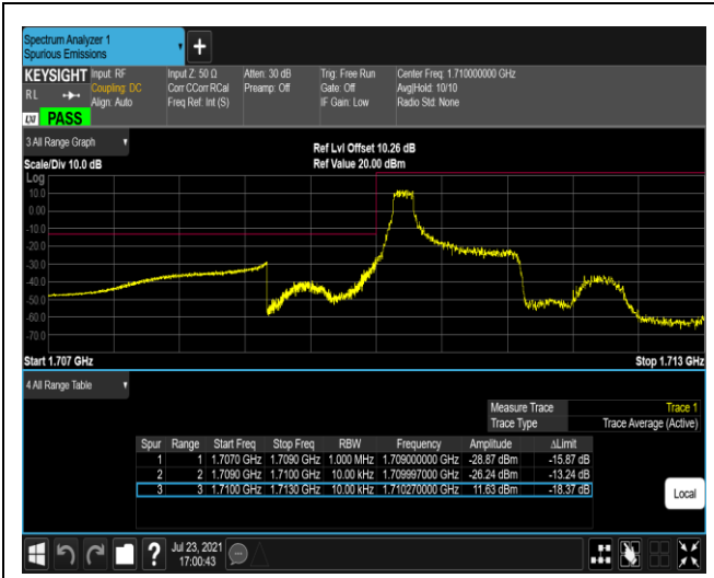
Band4-1.4MHz-16QAM-19957-1RB#0
