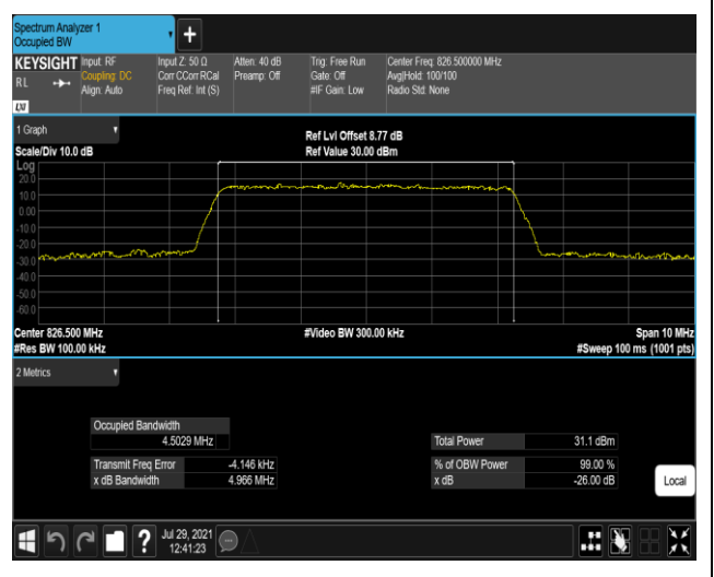
Band5-5MHz-16QAM-20425-25RB#0
