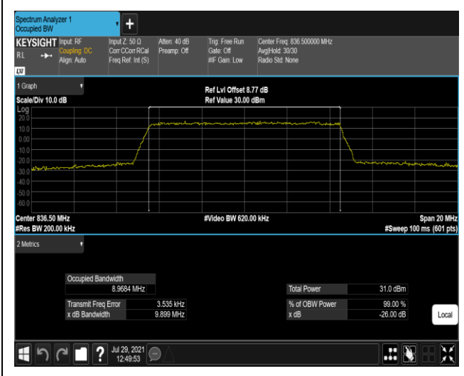
Band5-10MHz-16QAM-20525-50RB#0
