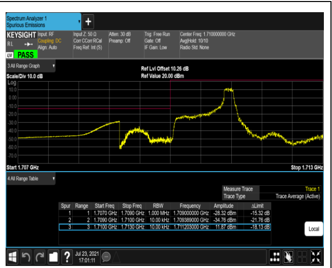
Band4-1.4MHz-16QAM-19957-1RB#5
