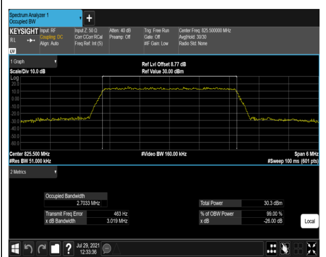
Band5-3MHz-16QAM-20415-15RB#0
