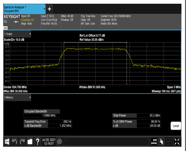
Band5-1.4MHz-16QAM-20407-6RB#0
