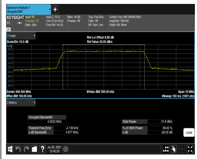
Band5-5MHz-QPSK-20625-25RB#0
