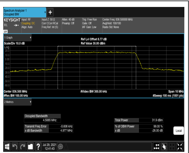
Band5-5MHz-QPSK-20525-25RB#0
