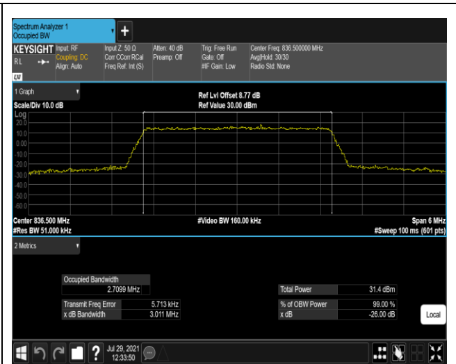
Band5-3MHz-QPSK-20525-15RB#0
