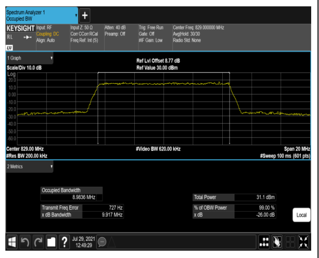
Band5-10MHz-16QAM-20450-50RB#0
