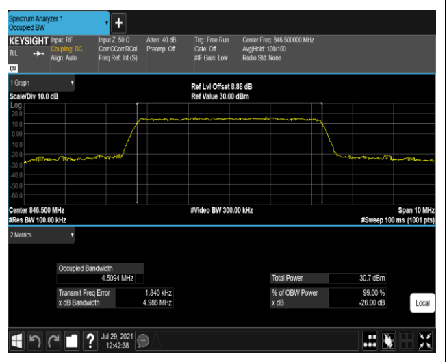
Band5-5MHz-16QAM-20625-25RB#0
