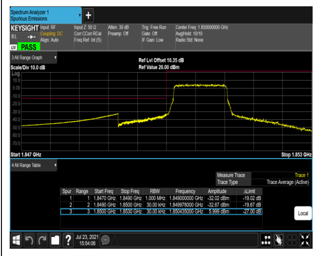
Band2-1.4MHz-16QAM-18607-6RB#0
