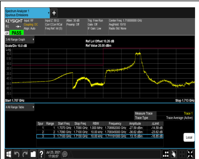
Band4-1.4MHz-QPSK-19957-1RB#5
