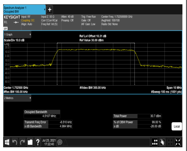
Band4-5MHz-16QAM-20375-25RB#0
