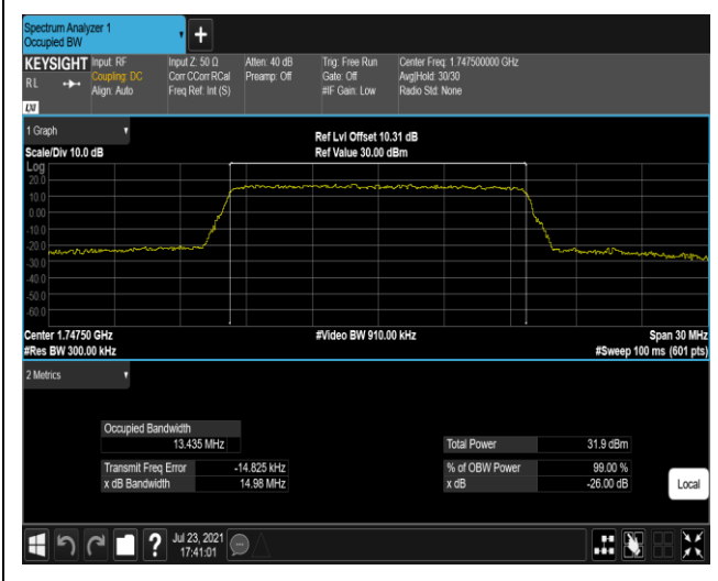
Band4-15MHz-QPSK-20325-75RB#0
