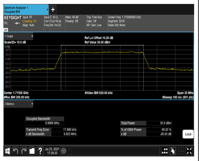
Band4-10MHz-16QAM-20000-50RB#0
