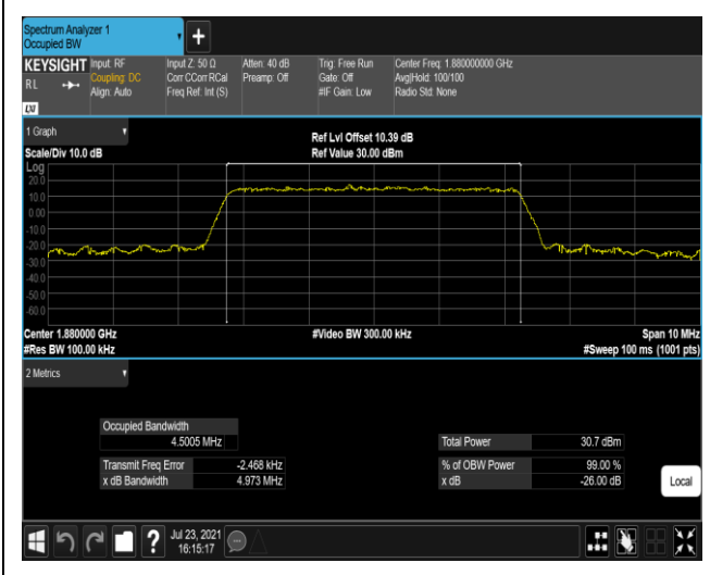
Band2-5MHz-16QAM-18900-25RB#0
