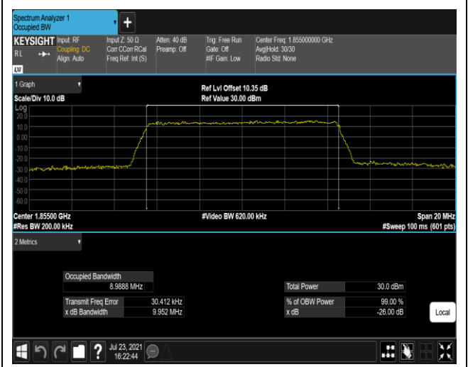
Band2-10MHz-16QAM-18650-50RB#0
