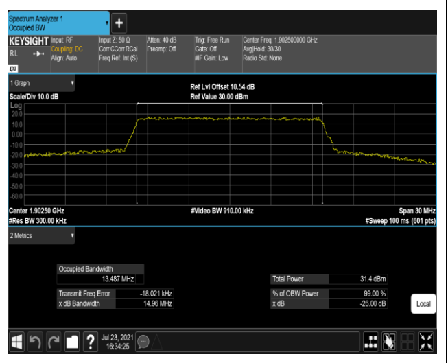
Band2-15MHz-16QAM-19125-75RB#0
