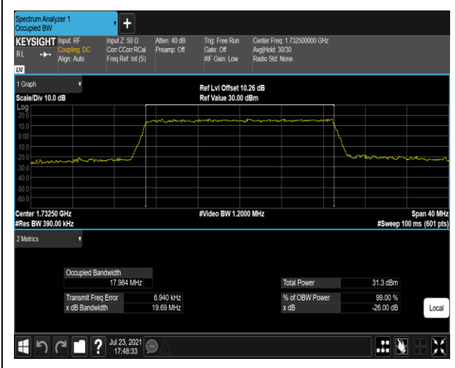
Band4-20MHz-16QAM-20175-100RB#0
