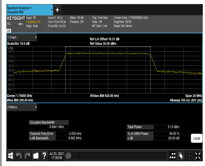
Band4-10MHz-QPSK-20350-50RB#0
