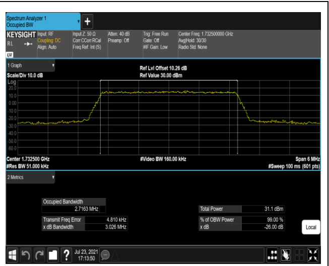
Band4-3MHz-QPSK-20175-15RB#0
