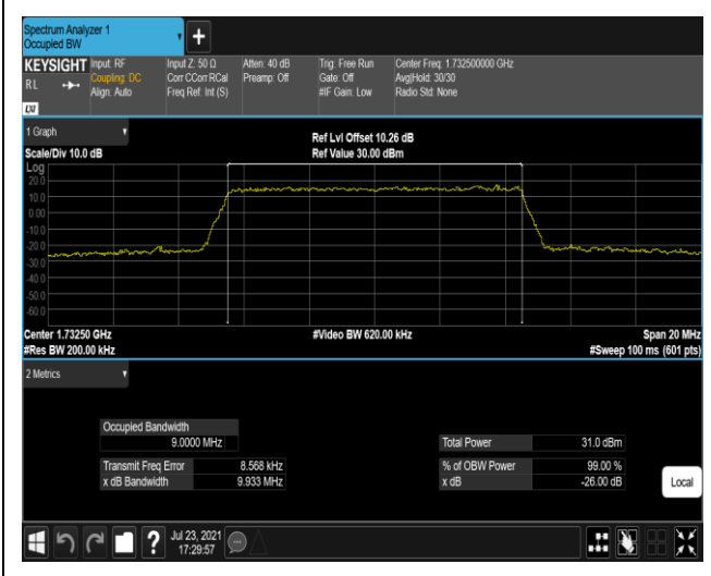
Band4-10MHz-16QAM-20175-50RB#0
