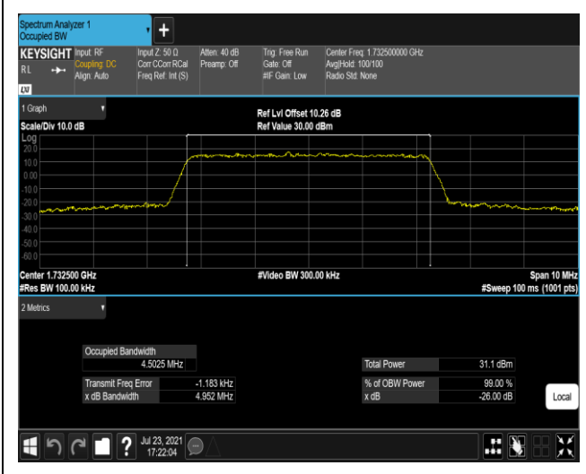
Band4-5MHz-16QAM-20175-25RB#0
