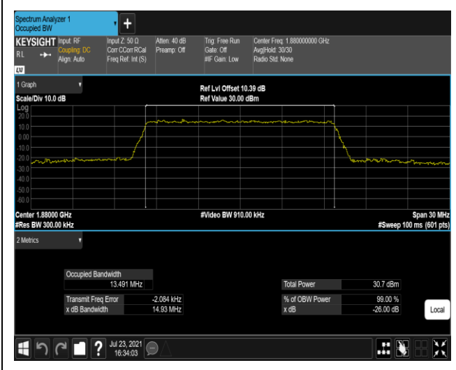
Band2-15MHz-16QAM-18900-75RB#0
