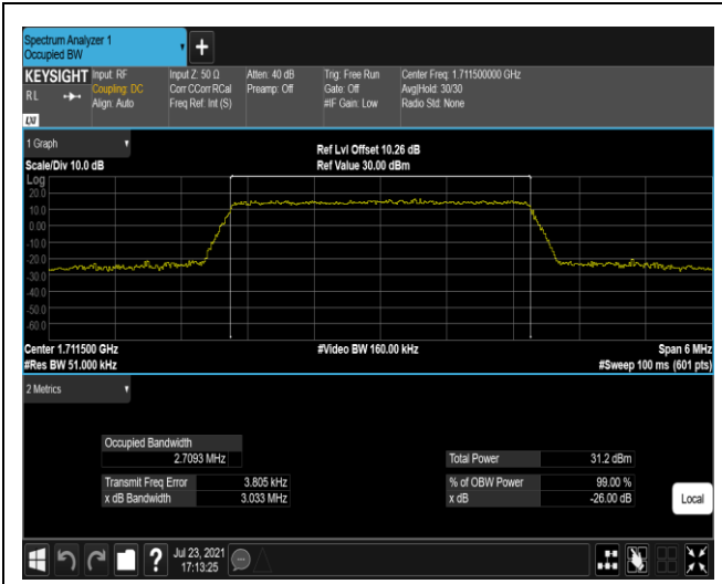
Band4-3MHz-QPSK-19965-15RB#0
