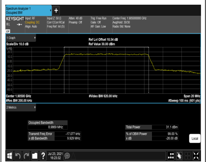
Band2-10MHz-16QAM-19150-50RB#0
