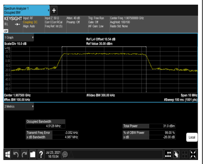
Band2-5MHz-16QAM-19175-25RB#0
