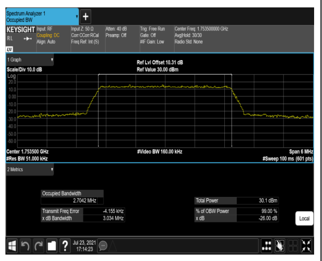
Band4-3MHz-16QAM-20385-15RB#0
