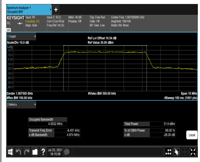
Band2-5MHz-QPSK-19175-25RB#0
