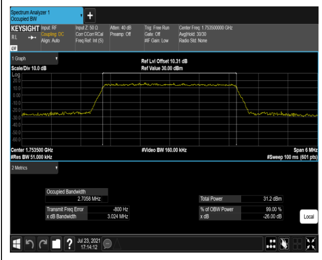
Band4-3MHz-QPSK-20385-15RB#0
