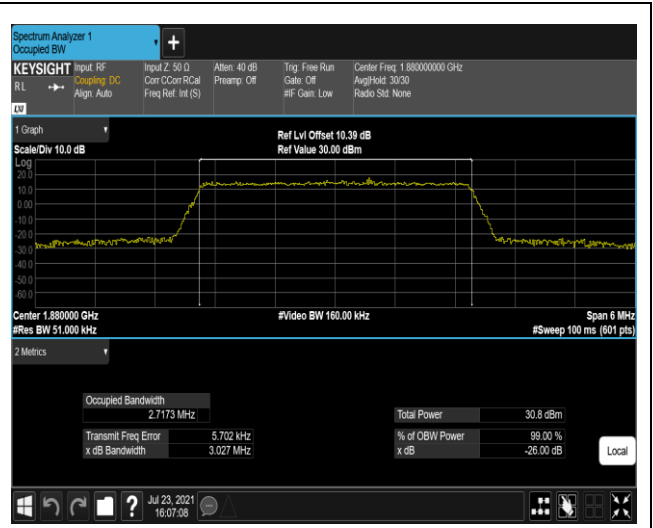
Band2-3MHz-QPSK-18900-15RB#0
