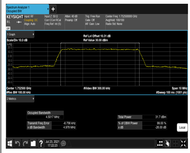
Band4-5MHz-QPSK-20375-25RB#0
