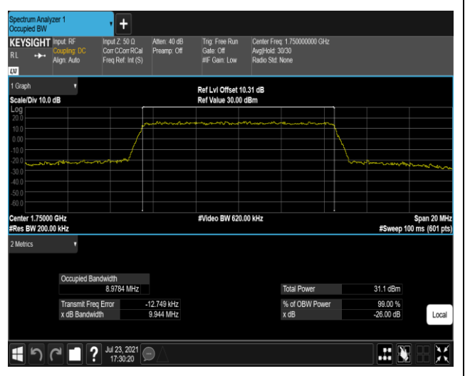
Band4-10MHz-16QAM-20350-50RB#0
