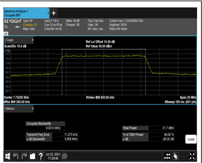
Band4-10MHz-QPSK-20175-50RB#0
