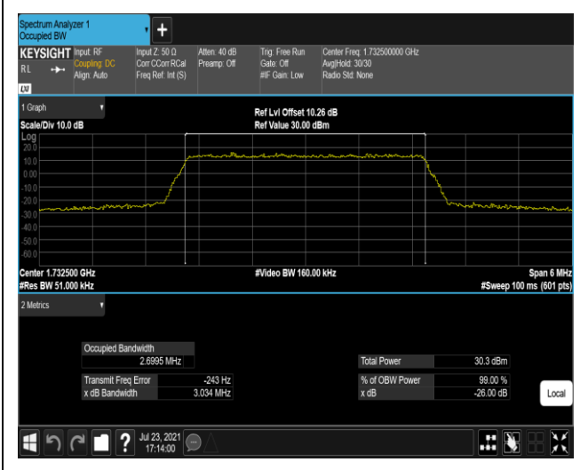
Band4-3MHz-16QAM-20175-15RB#0
