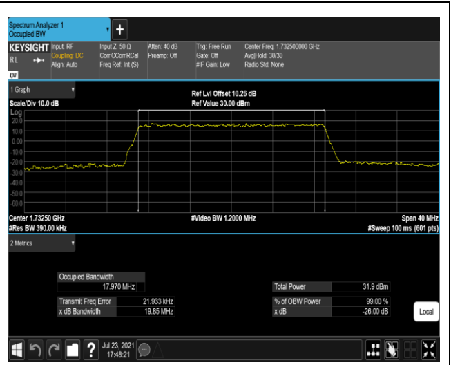
Band4-20MHz-QPSK-20175-100RB#0
