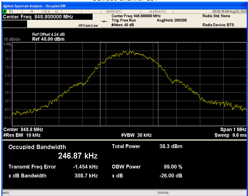
GSM850 Channel=251
