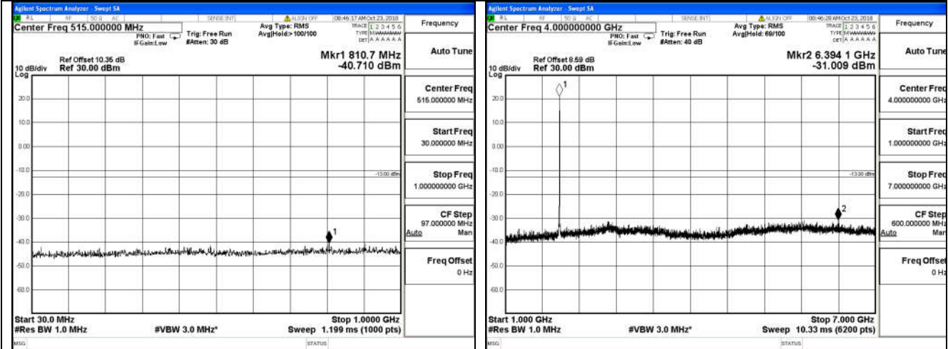
30 MHz – 1000 MHz
