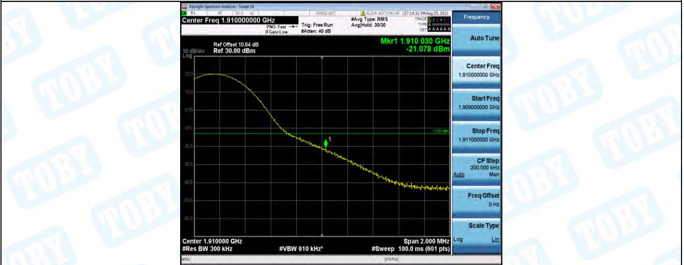
Band2-15MHz-16QAM-19125-75RB#0
