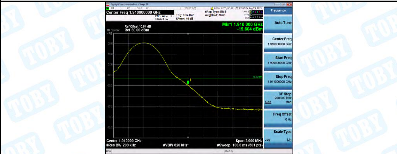
Band2-10MHz-QPSK-19150-50RB#0
