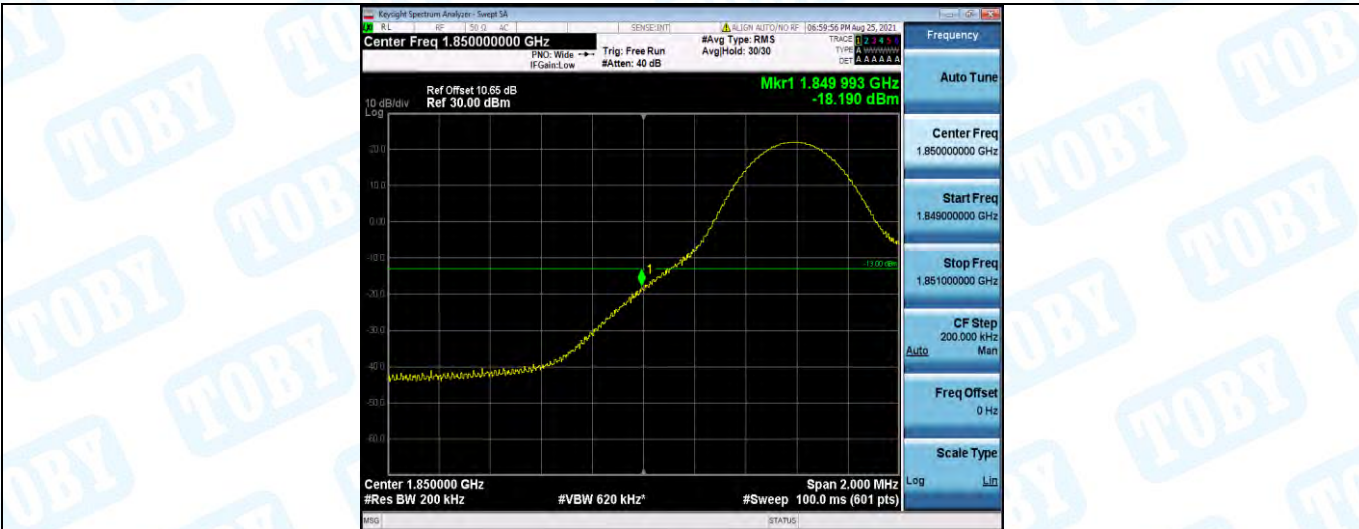
Band2-10MHz-QPSK-18650-1RB#49
