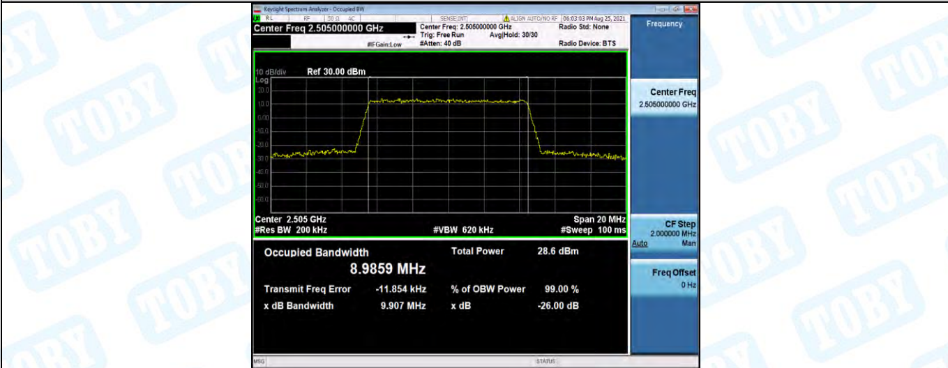
Band7-10MHz-16QAM-2100-50RB#0
