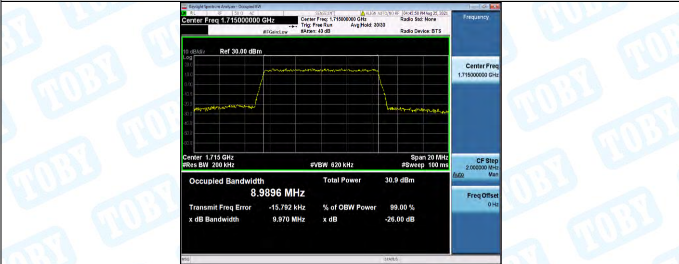
Band4-10MHz-16QAM-20175-50RB#0
