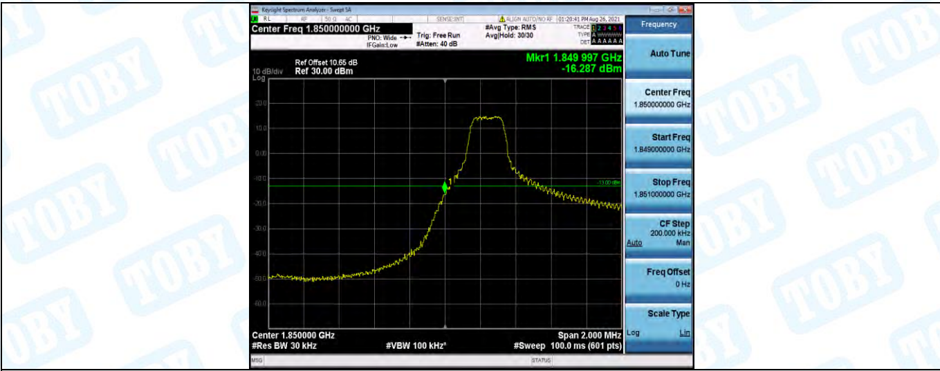
Band2-3MHz-16QAM-18615-1RB#14
