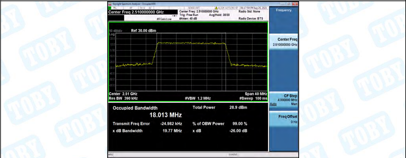
Band7-20MHz-16QAM-21100-100RB#0
