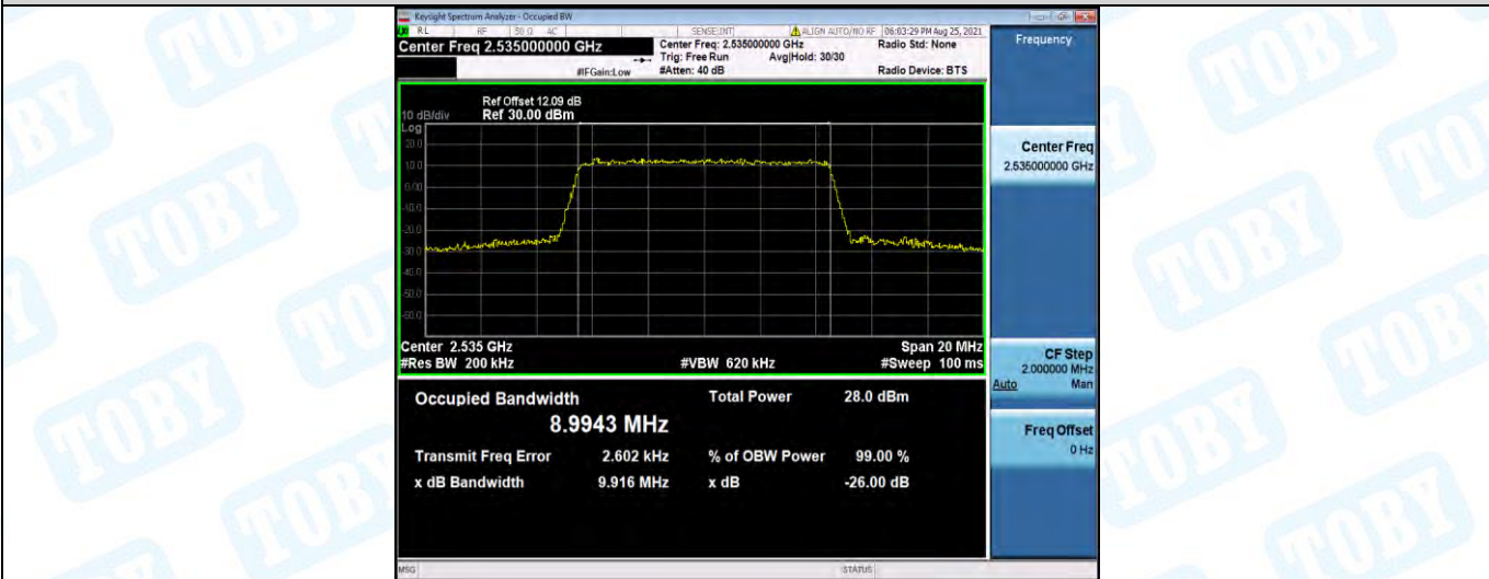
Band7-10MHz-16QAM-21400-50RB#0
