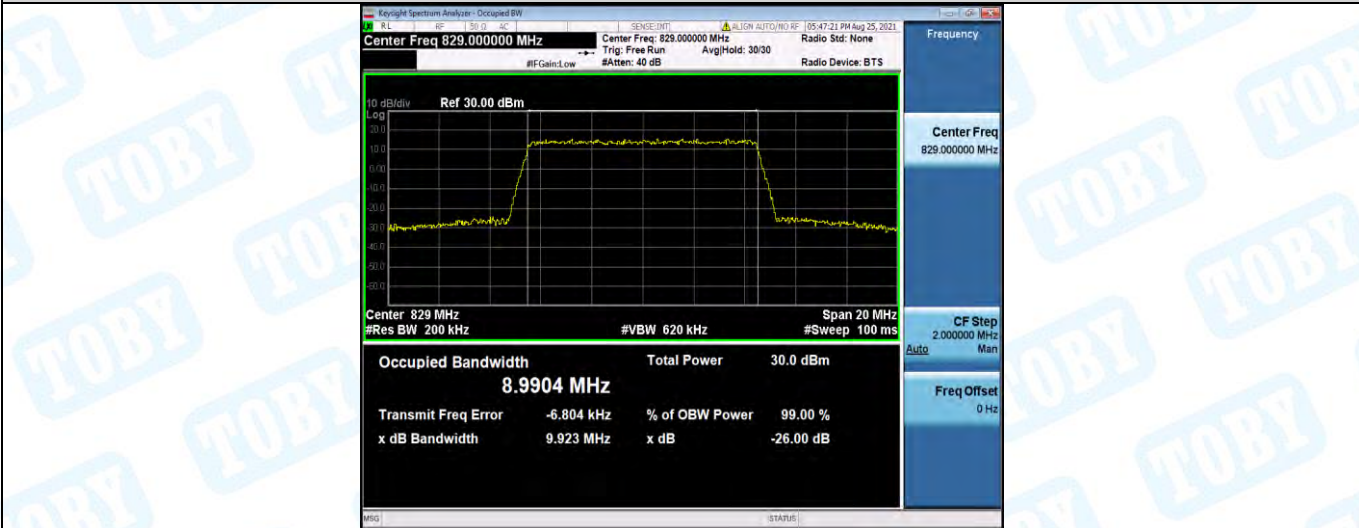
Band5-10MHz-16QAM-20525-50RB#0
