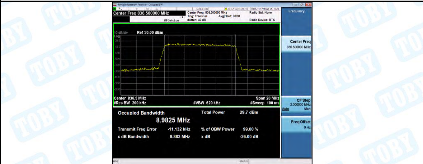
Band5-10MHz-16QAM-20600-50RB#0
