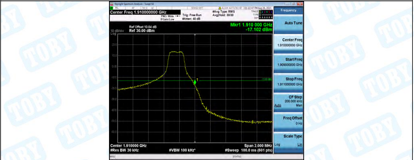
Band2-3MHz-16QAM-19185-15RB#0
