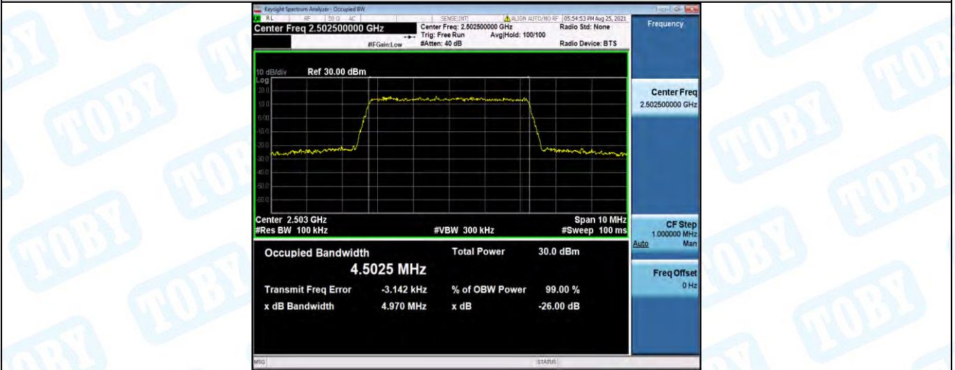
Band7-5MHz-QPSK-21100-25RB#0
