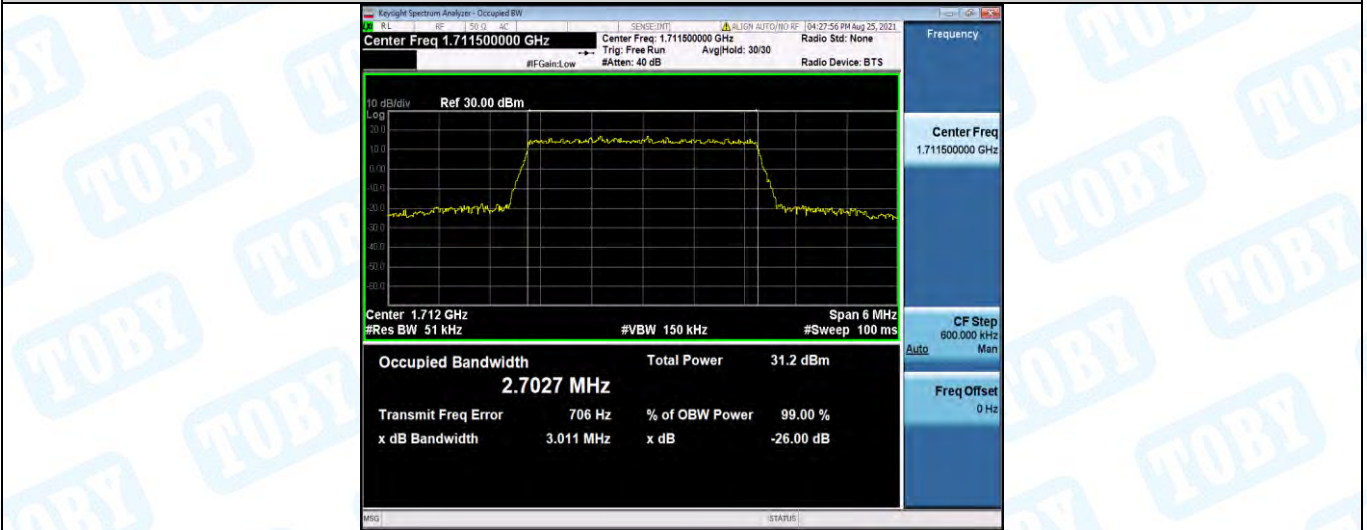
Band4-3MHz-QPSK-20175-15RB#0
