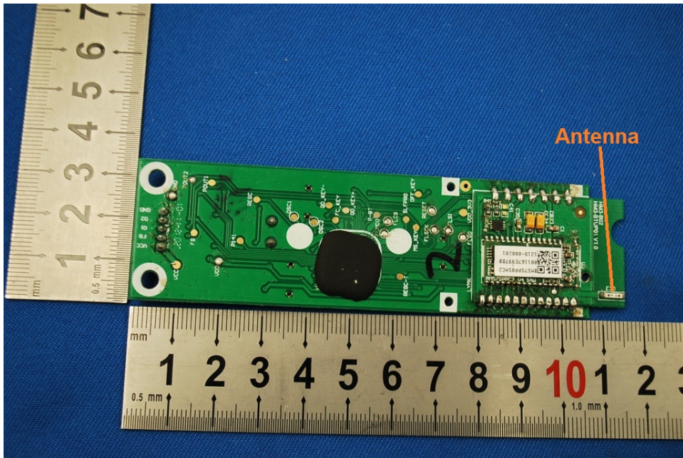
Control PCB Front View
