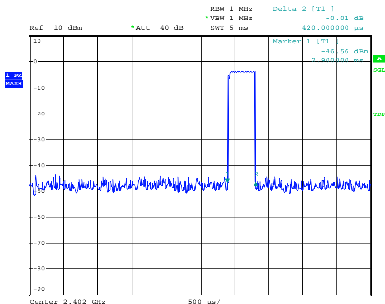
Figure 13: Dwell Time, Mode E (Hopping), DH1, Low channel
