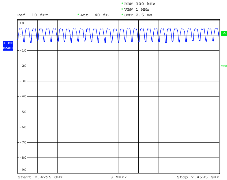
Figure 11: Hopping Frequencies up to 2459.5MHz, Mode E (Hopping)
