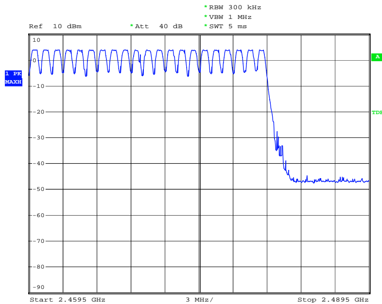
Figure 12: Hopping Frequencies up to 2489.5MHz, Mode E (Hopping)
