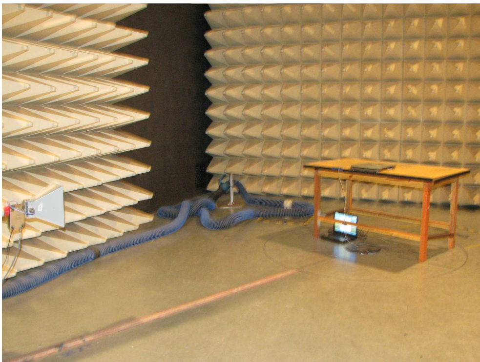
Photograph 5: Set-up for Radiated Emission, 1G-18GHz
