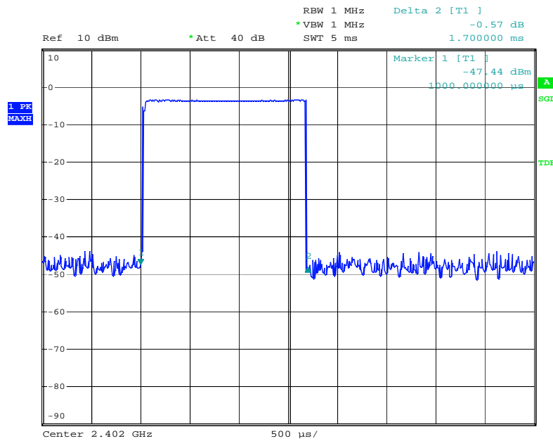
Figure 14: Dwell Time, Mode E (Hopping), DH3, Low channel
