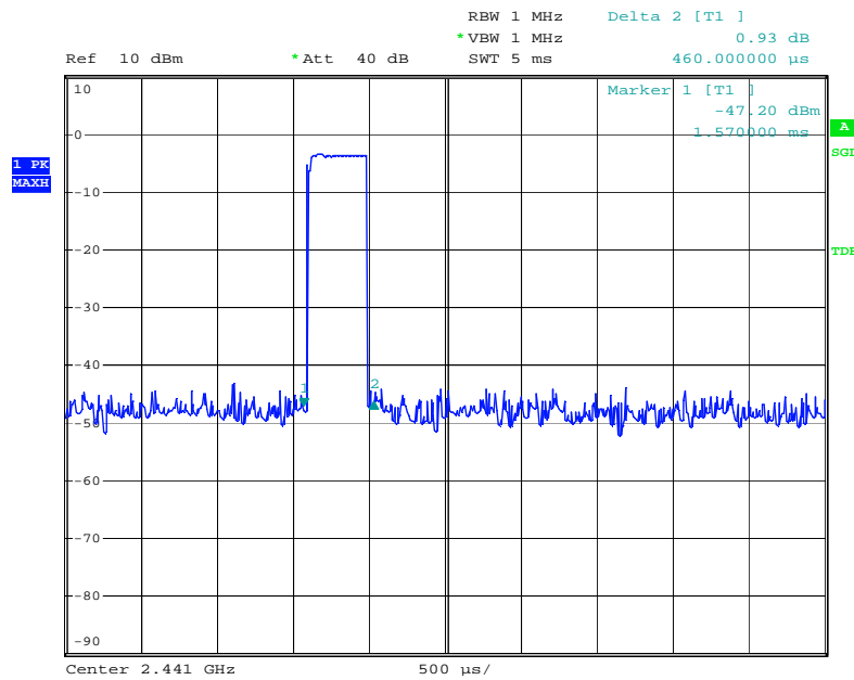
Figure 16: Dwell Time, Mode E (Hopping), DH1, Mid channel
