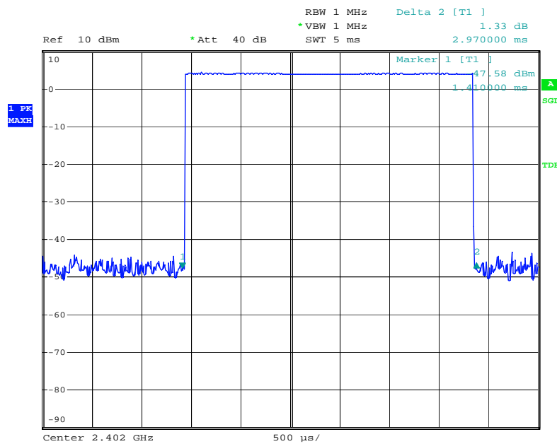
Figure 15: Dwell Time, Mode E (Hopping), DH5, Low channel
