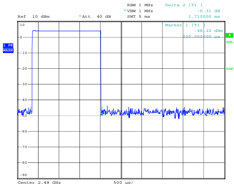
Figure 20: Dwell Time, Mode E (Hopping), DH3, High channel
