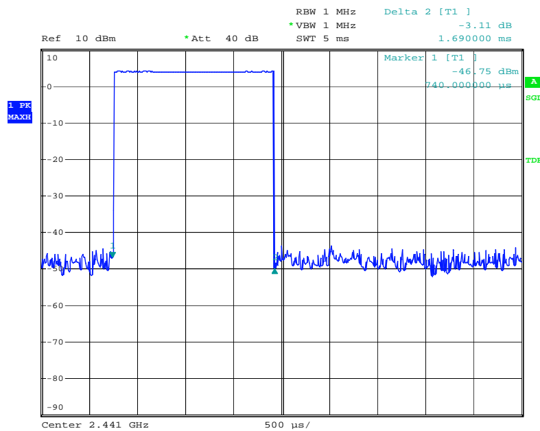
Figure 17: Dwell Time, Mode E (Hopping), DH3, Mid channel
