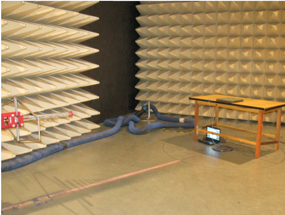
Photograph 4: Set-up for Set-up for Radiated Emission, 30MHz-1000MHz
