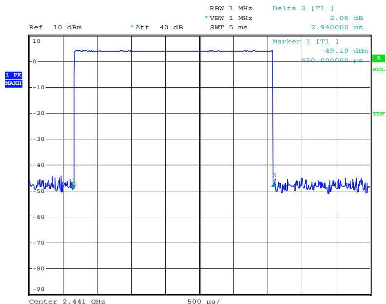
Figure 18: Dwell Time, Mode E (Hopping), DH5, Mid channel
