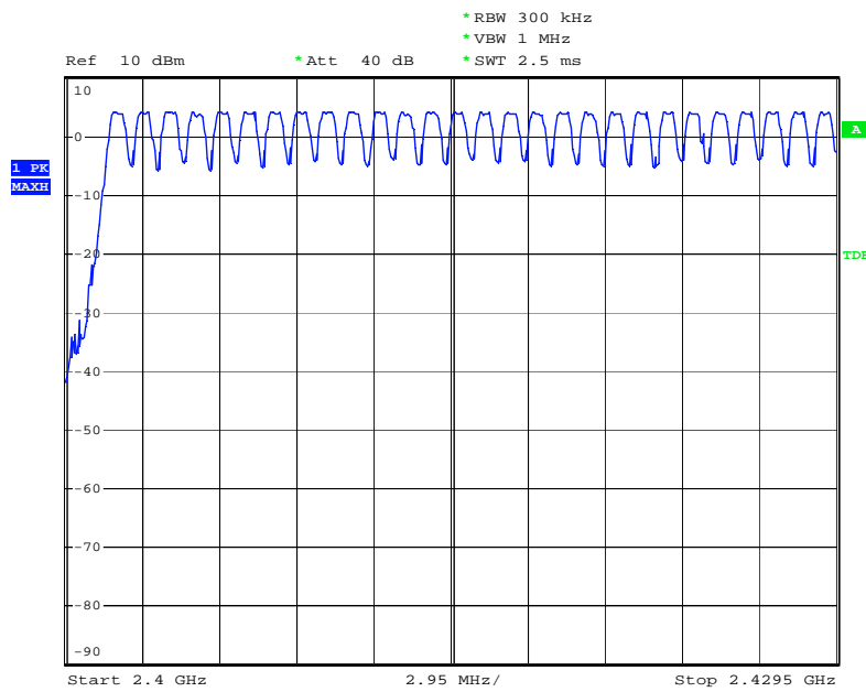
Figure 10: Hopping Frequencies up to 2429.5MHz, Mode E (Hopping)
