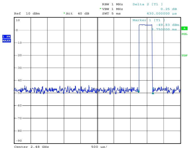
Figure 19: Dwell Time, Mode E (Hopping), DH1, High channel
