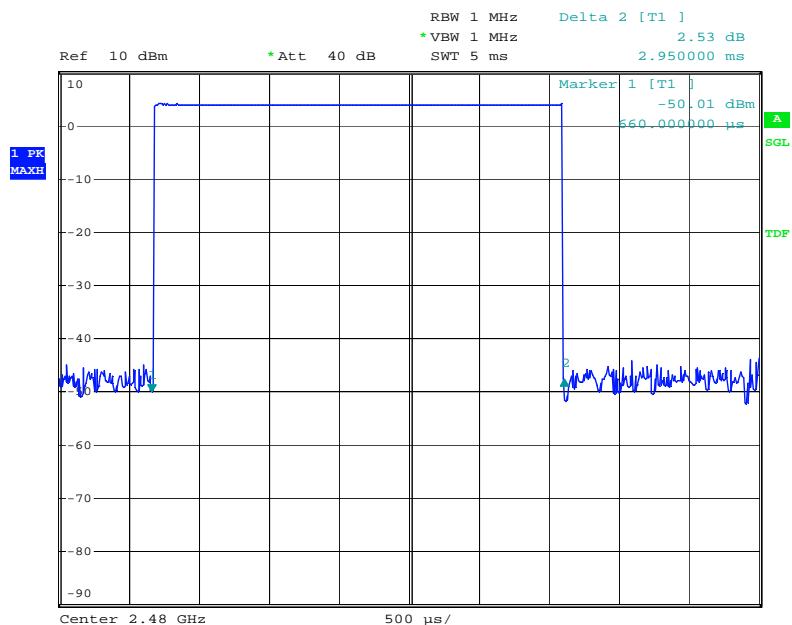
Figure 21: Dwell Time, Mode E (Hopping), DH5, High channel
