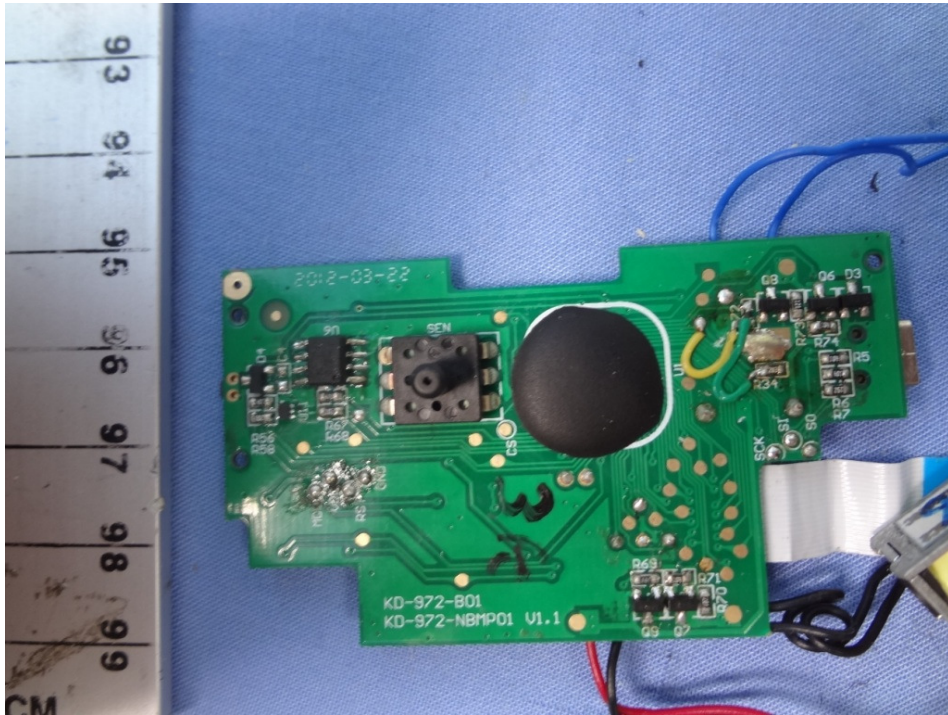
Power Board Rear View
