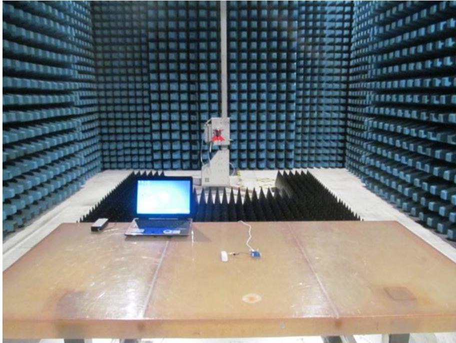
Photograph 3: Set-up for Conduct Power
