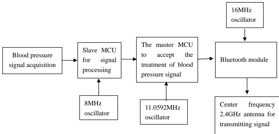
KD-923 Blood pressure monitor frequency diagram
