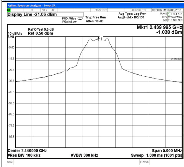
BT LE-Middle channel Reference
