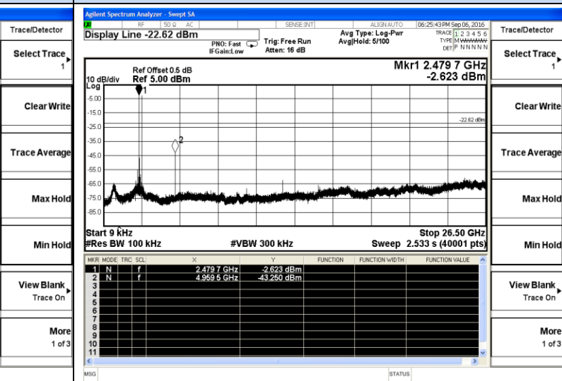
BT LE-High channel
