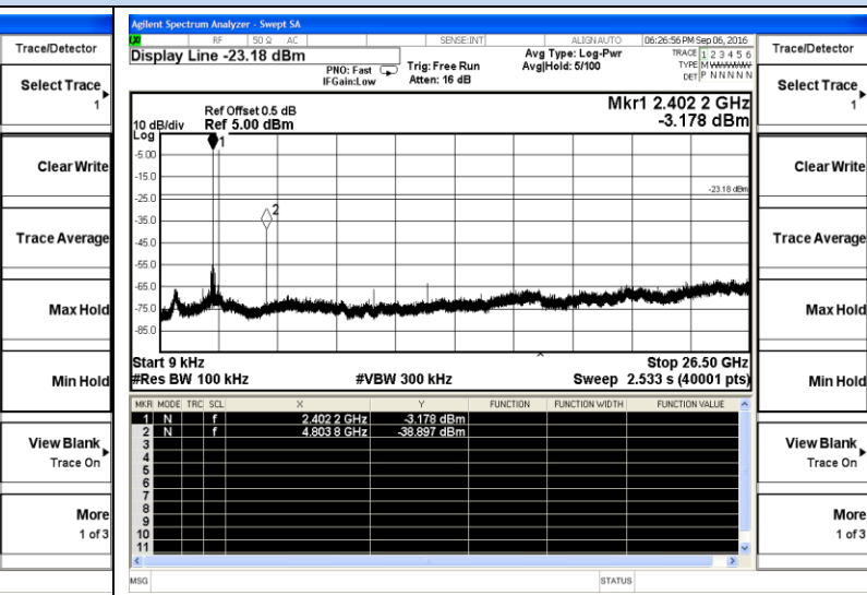
BT LE-Low channel
