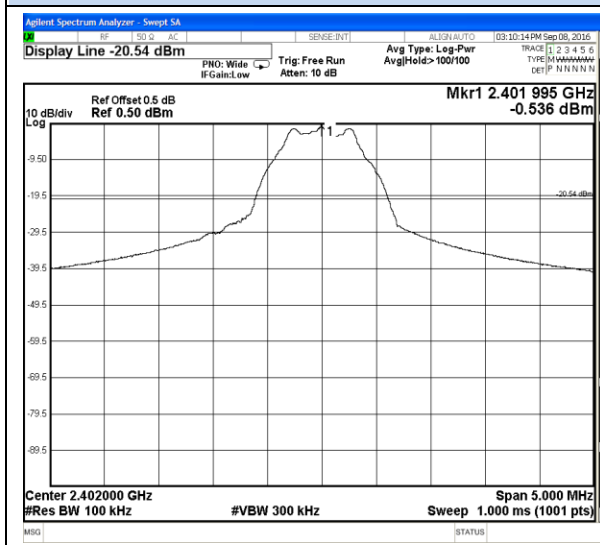
BT LE-Low channel Reference
