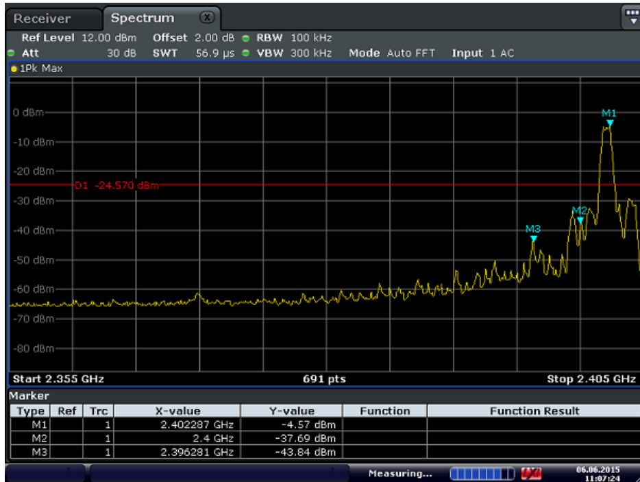
(1Mbps) The Lowest Channel 00: 2402MHz
