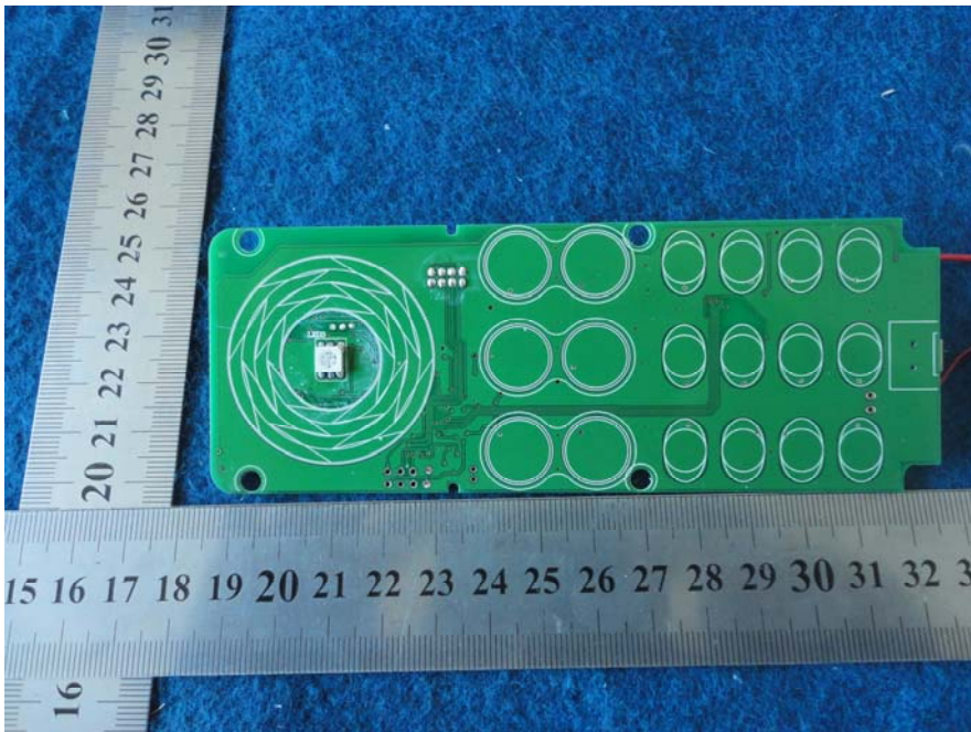
PCB photograph of Transmitter
