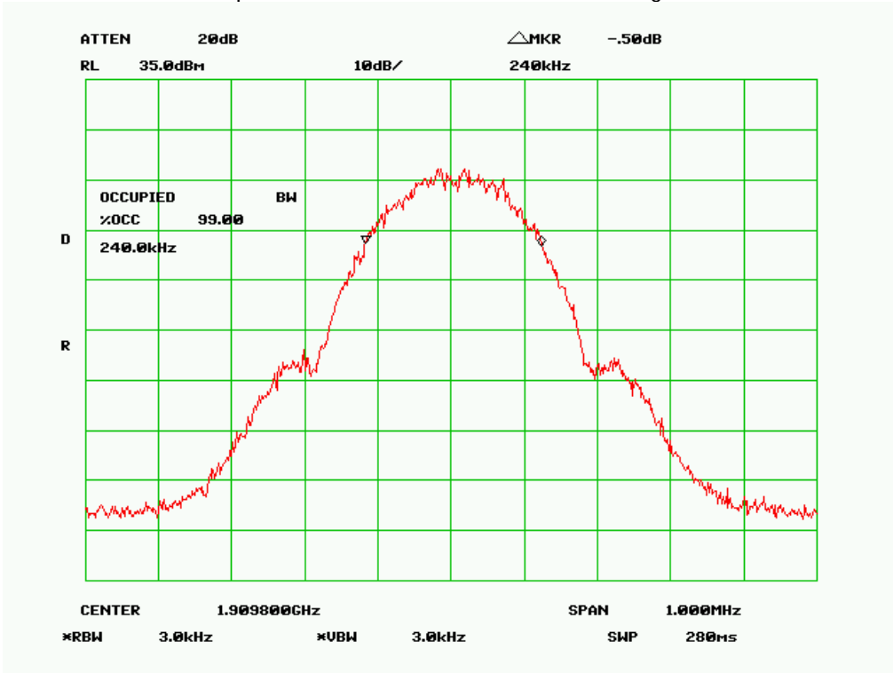
99% Occupied Bandwidth –GPRS1900, Channel 810, High Channel
