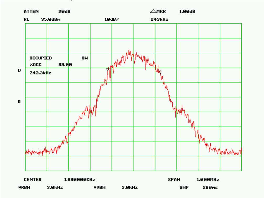
99% Occupied Bandwidth – GPRS1900, Channel 661, Mid Channel
