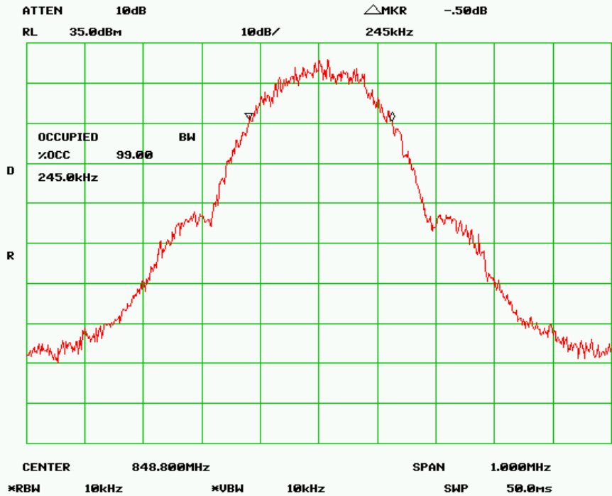
99% Occupied Bandwidth –EGPRS850, Channel 251, High Channel
