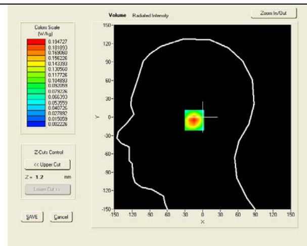
SAR, Z Axis Scan (X = -10, Y = -5)
