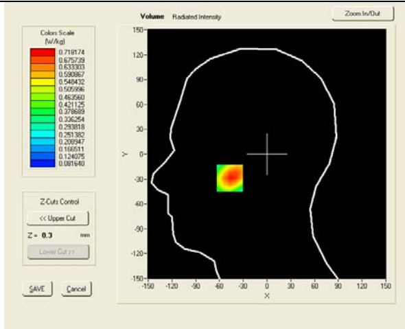
SAR, Z Axis Scan (X = -47, Y = -29)
