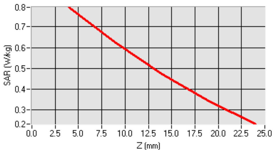
SAR, Z Axis Scan (X = -35, Y = -17)
