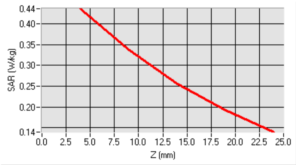
SAR, Z Axis Scan (X = -31, Y = -15)
