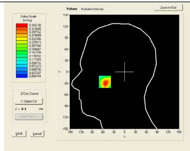
SAR, Z Axis Scan (X = -54, Y = -26)
