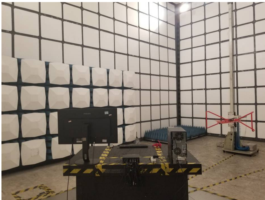
Back View of Radiated Emission Test (30MHz ~ 1GHz)
