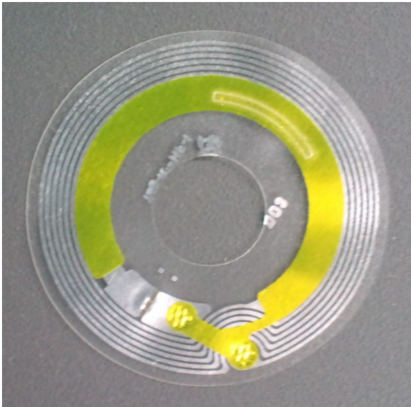
IC_Tag(Front side)
