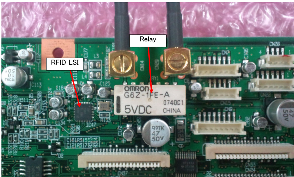
Radio Unit (Front side)
