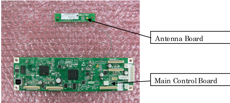
Antenna Board(Front side)
