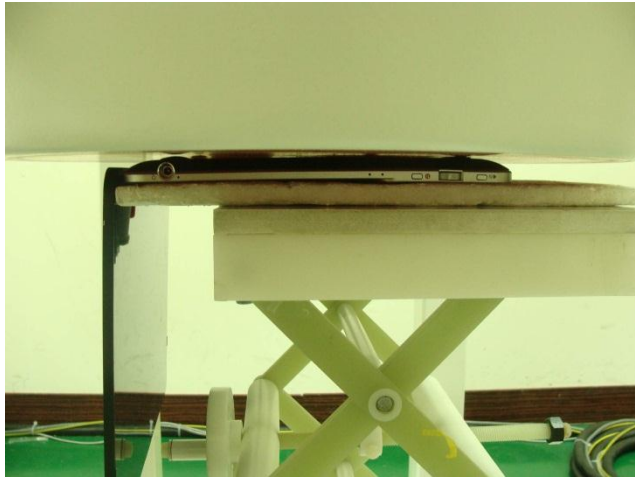
Bottom of the DUT with Phantom 0 cm Gap (Sample 2 with Battery 2)
