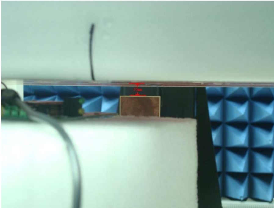
Figure 4. Body SAR Test Setup (Flat Section) _ Side D
