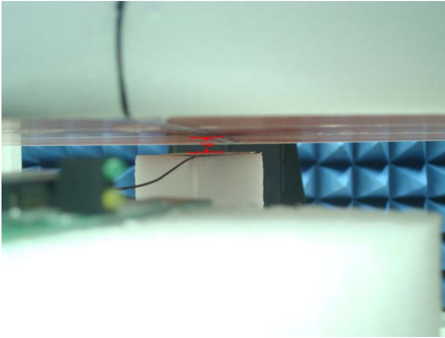
Figure 1. Body SAR Test Setup (Flat Section) _ Side A
