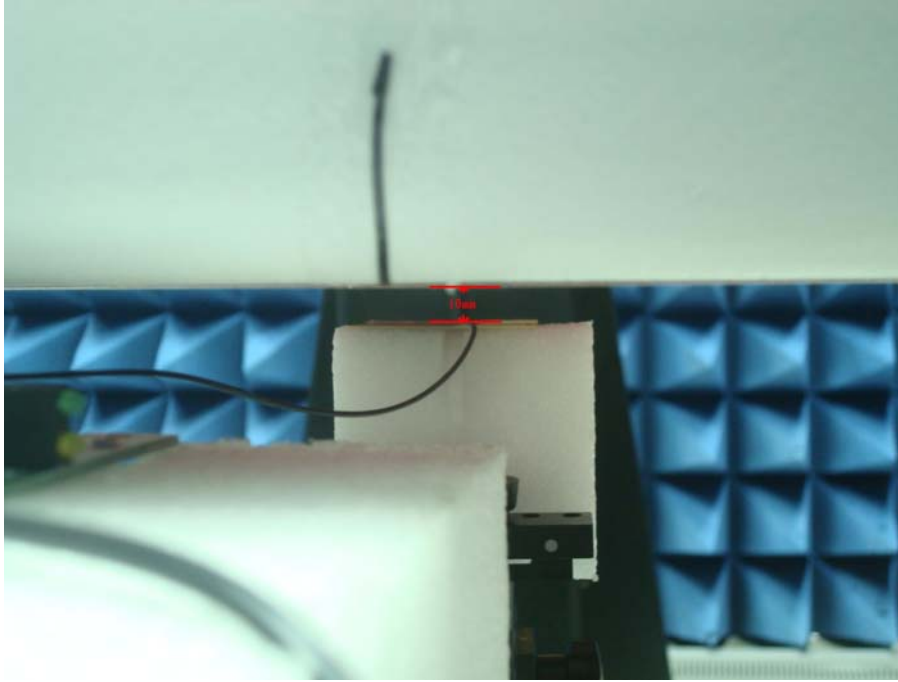
Figure 2. Body SAR Test Setup (Flat Section) _ Side B
