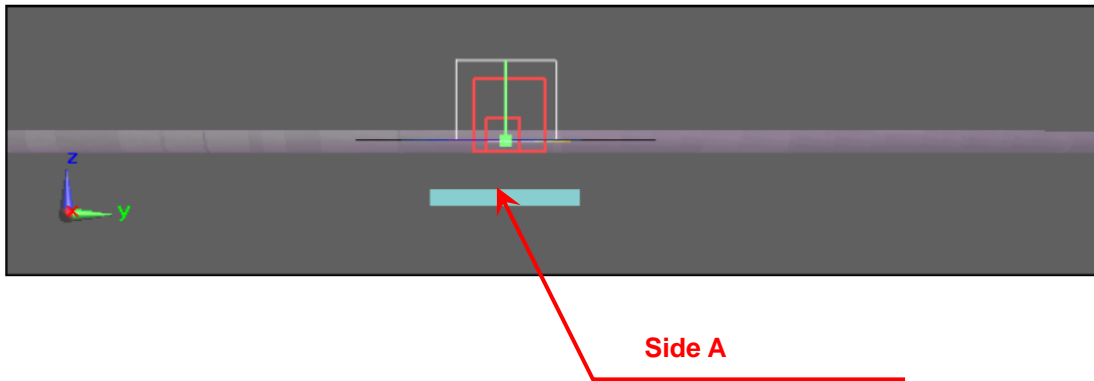
Figure 1. Body SAR Test Setup (Flat Section) _ Side A
