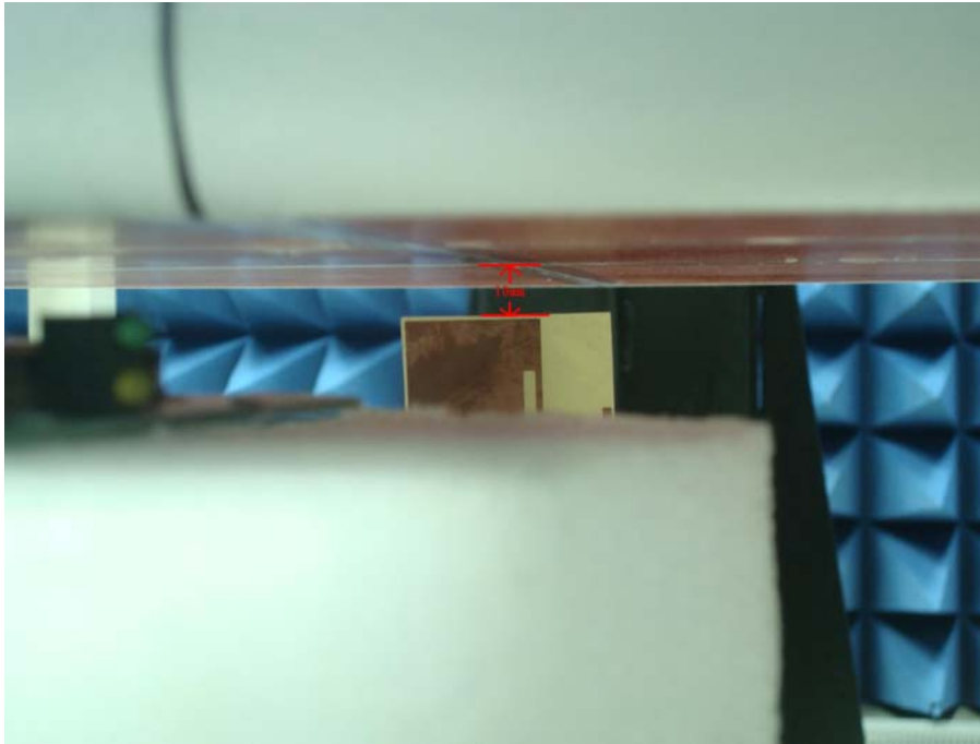
Figure 3. Body SAR Test Setup (Flat Section) _ Side C
