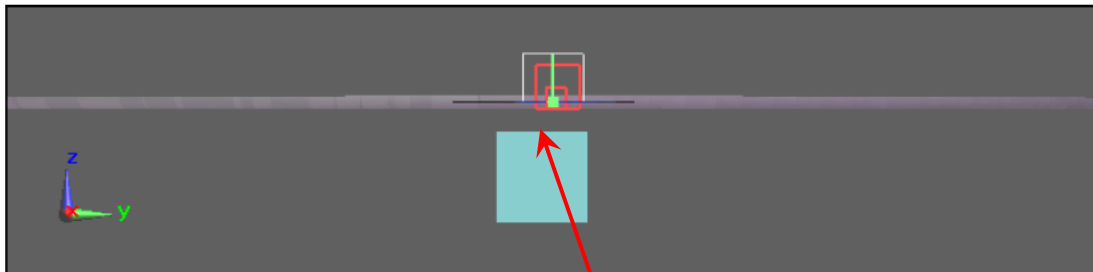
Figure 3. Body SAR Test Setup (Flat Section) _ Side C
