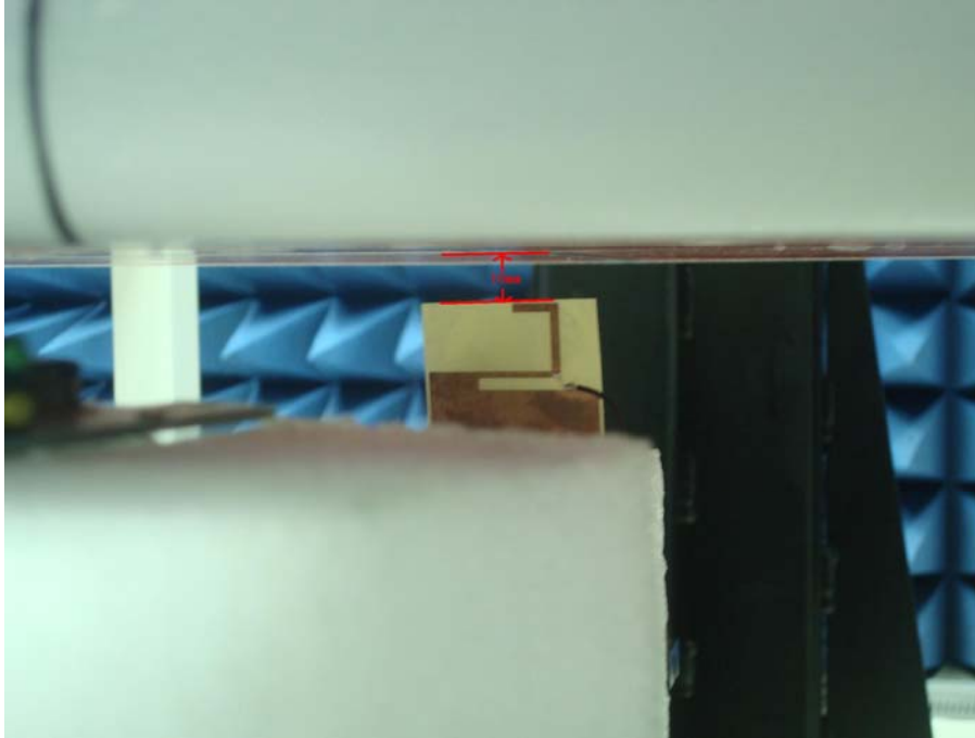
Figure 6. Body SAR Test Setup (Flat Section) _ Side F
