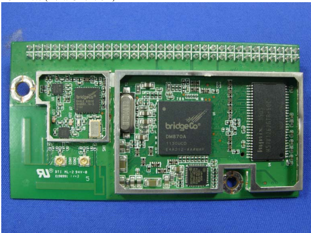
(6) EUT Photo (M/N: CX870-3H)
