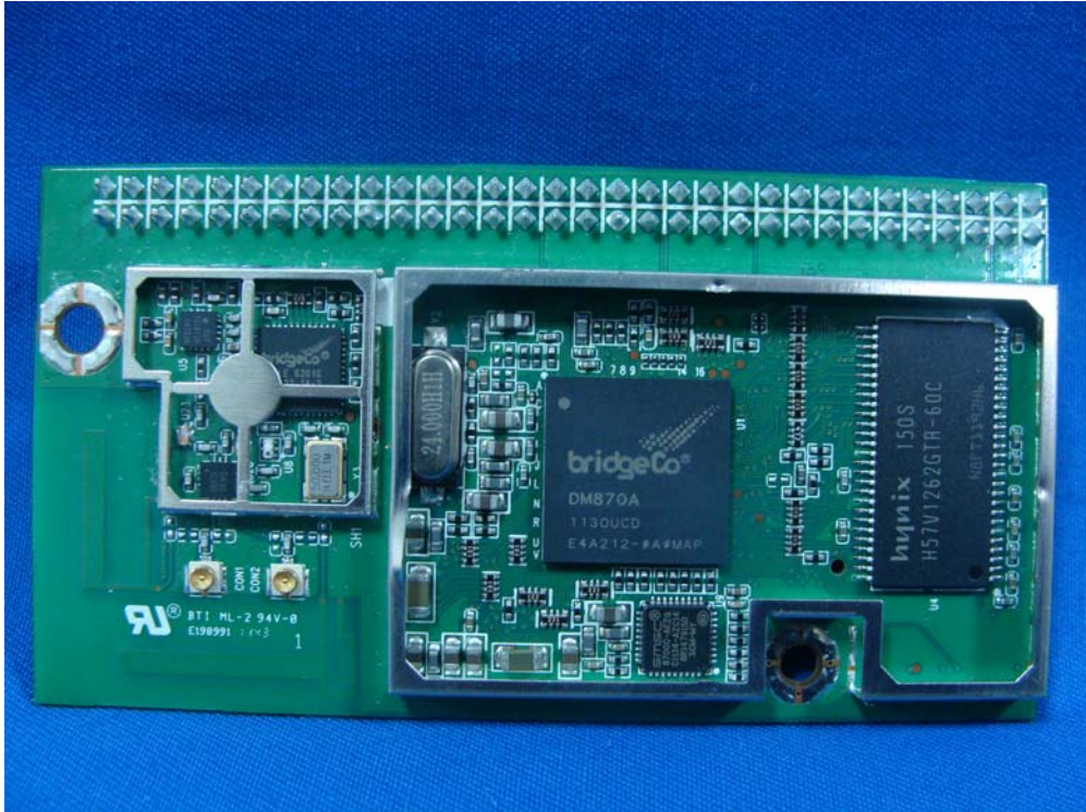
(9) EUT Photo (M/N: CX870-3HB)
