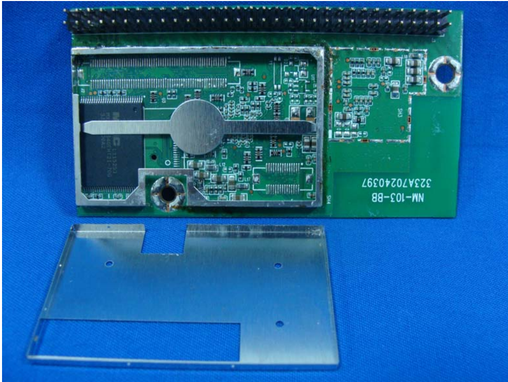
(11) EUT Photo (M/N: CX870-3HB)
