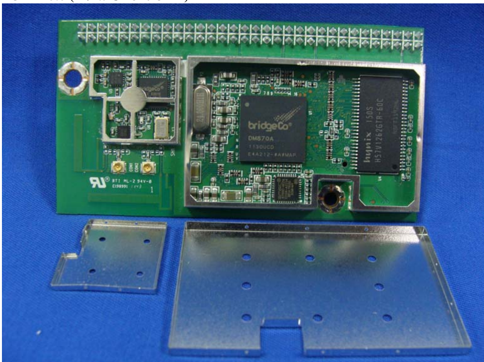
(8) EUT Photo (M/N: CX870-3HB)
