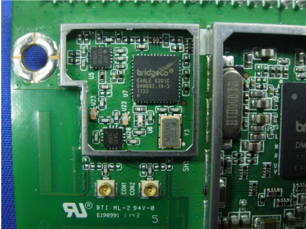
(7) EUT Photo (M/N: CX870-3H)
