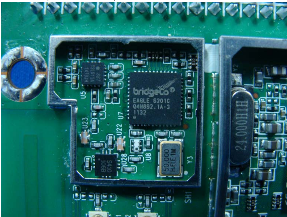
(10) EUT Photo (M/N: CX870-3HB)
