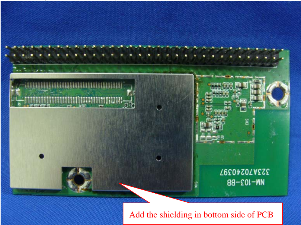
(4) EUT Photo (M/N: CX870-3HB)
