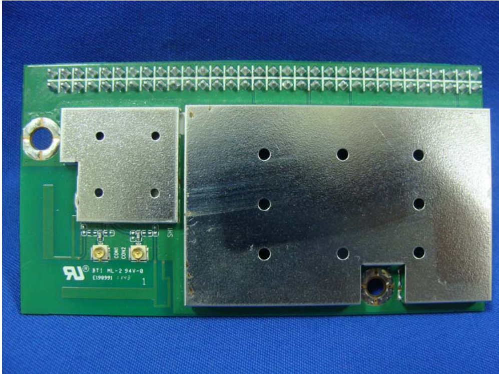
(3) EUT Photo (M/N: CX870-3HB)
