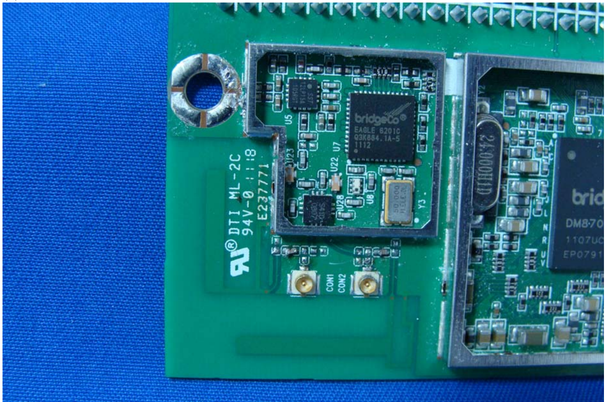
(7) EUT Photo
