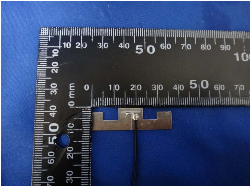
(16) EUT Photo_ MSA-3608-2G4C4-A2_B(Black 230mm)(ANT4-2)
