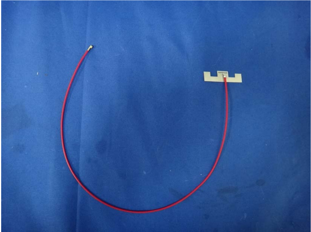
(14) EUT Photo_ MSA-3808-2G4C4-A4_B(Red 350mm)(ANT4-2)
