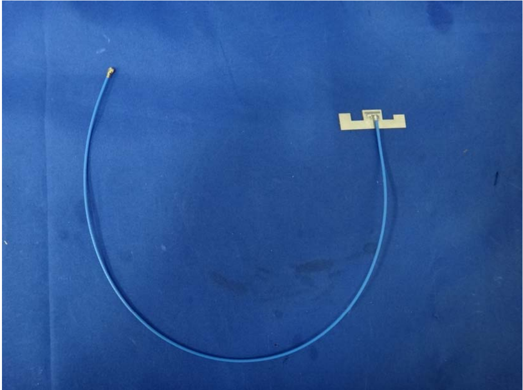
(18) EUT Photo_ MSA-3808-2G4C4-A2_B(Blue 350mm)
