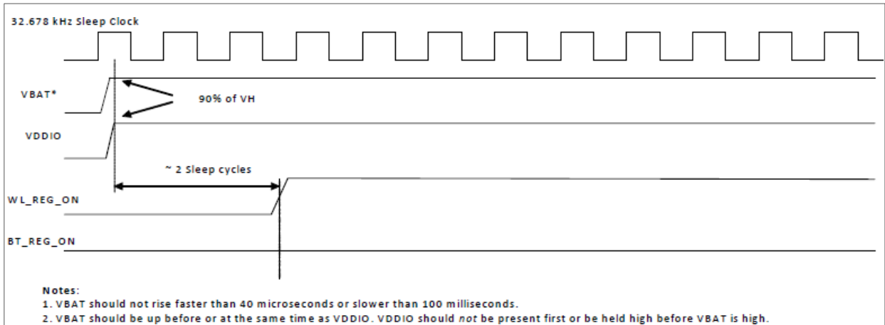
WLAN=ON, Bluetooth=OFF
